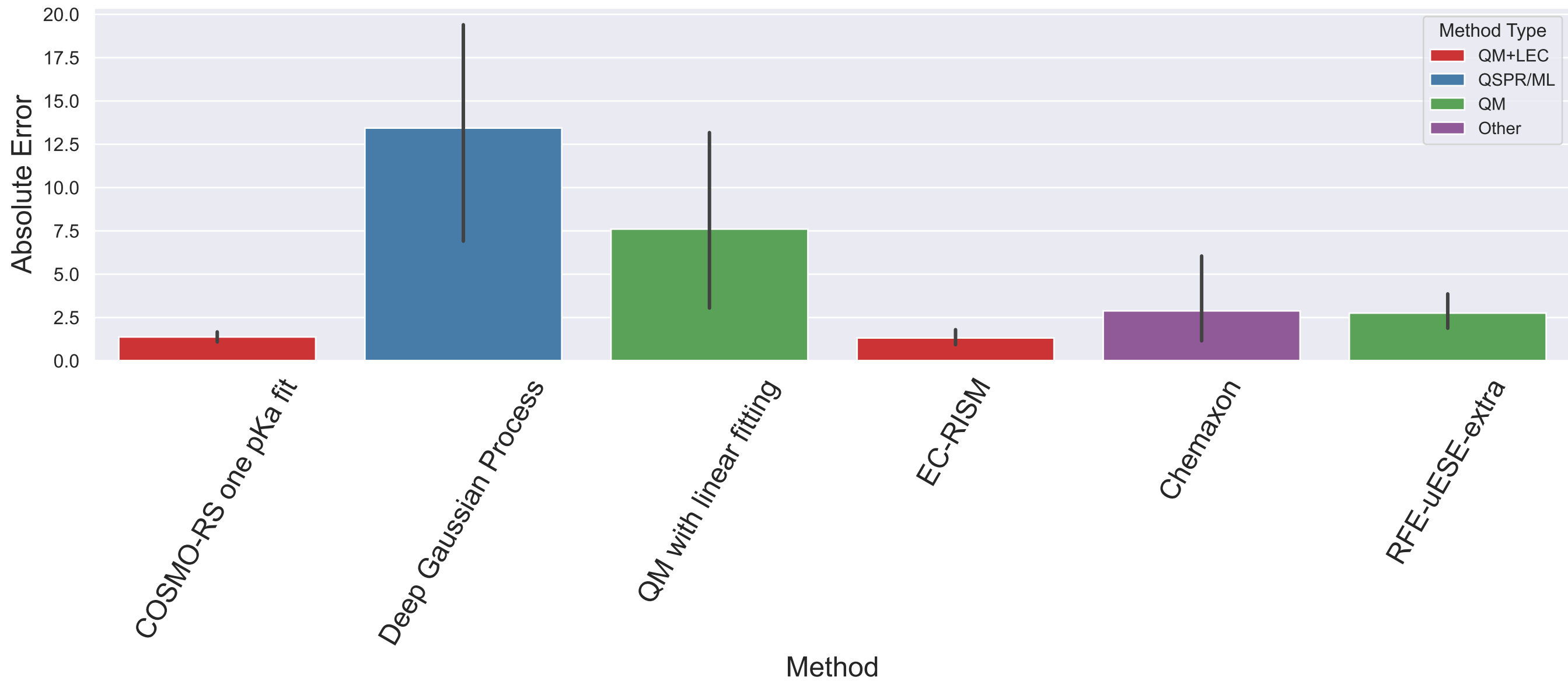
Absolute Error Based on Method
