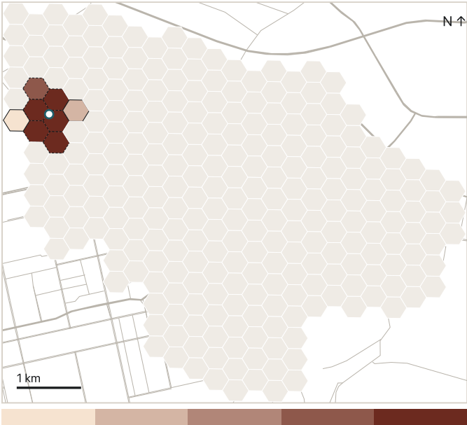
Lower priority → highest priority, within Landhi. Circle: where OpenStreetMap marks Allah Buksh Goth. Grey: the rest of Landhi. Lines: main roads.
