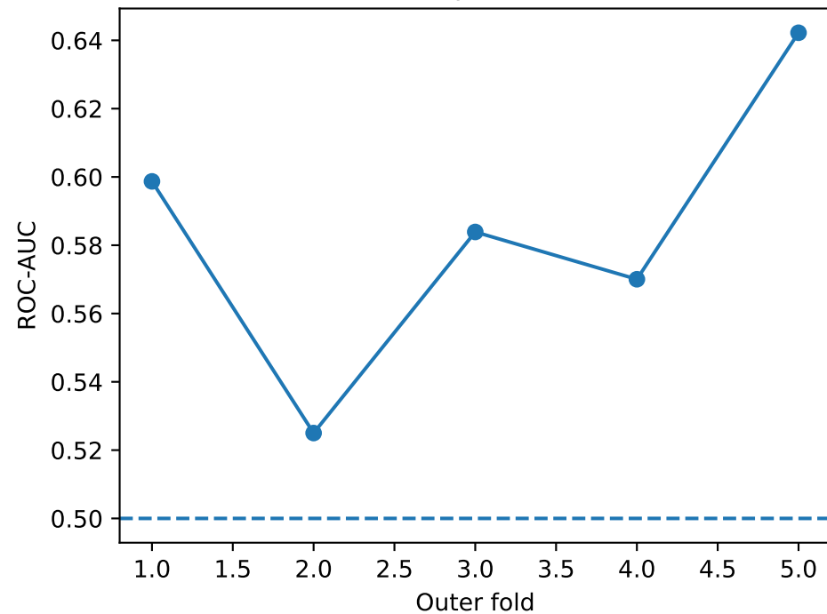
5-fold ML performance
