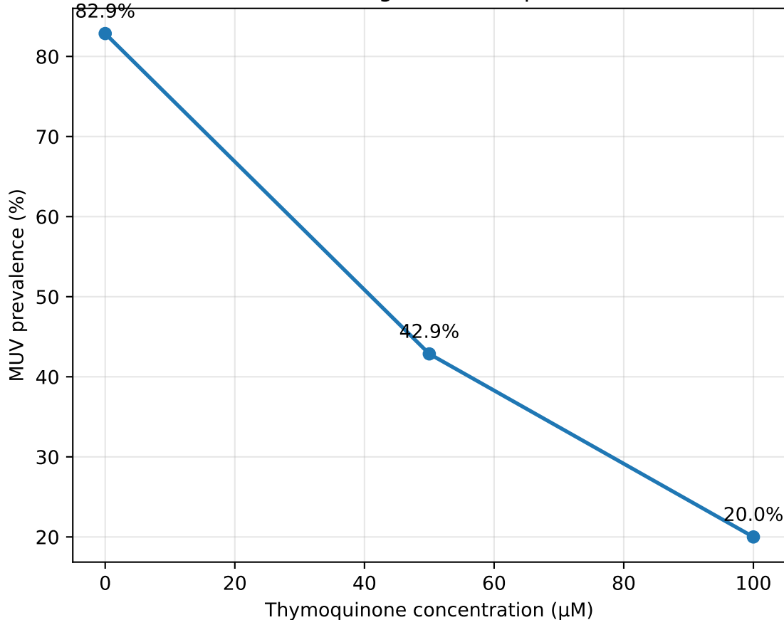
Cochran-Armitage Dose-Response Trend
