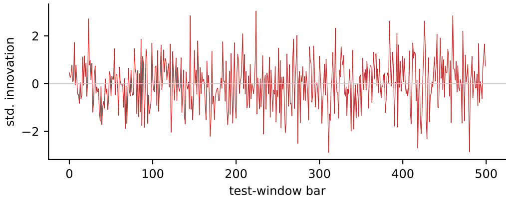
Independent random walk pair: Kalman innovations
