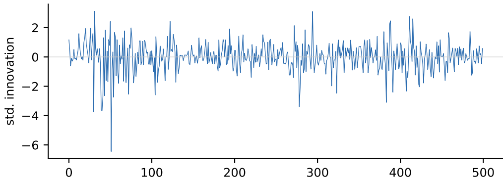
Independent random walk pair: Kalman innovations
