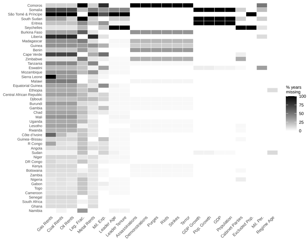
Figure B1. Pattern of Missing Data across Countries and Predictor Variables
