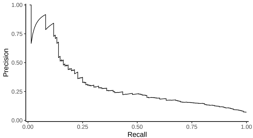
Figure E3. Precision Recall Curve for the Random Forest Model for Predicting Coup Attempts
