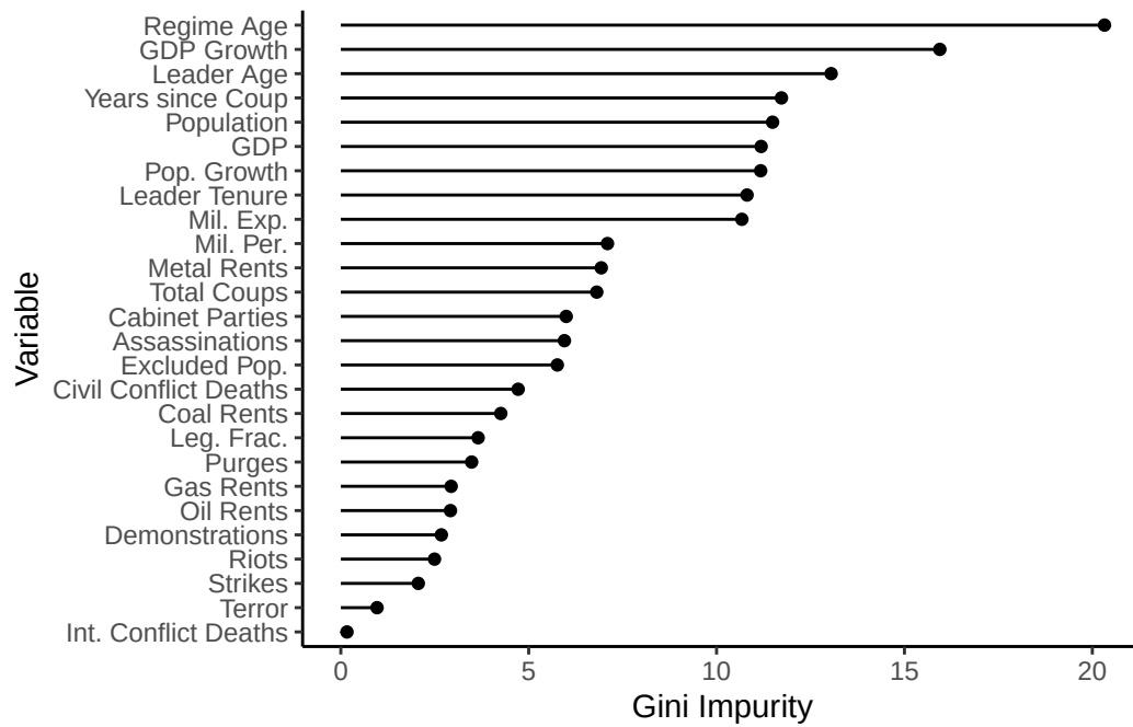
Figure E2. Importance of Variables in the Random Forest Model for Predicting Coup Attempts
