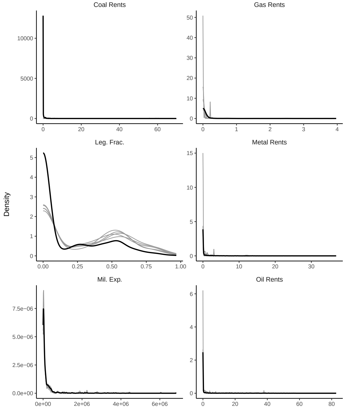
Figure B2. Observed vs. Imputed Distributions for Most-Missing Variables
