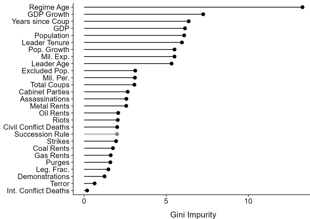
Figure C1. Importance of Variables in the Random Forest Model for Predicting Coups with Succession Rules as a Predictor
