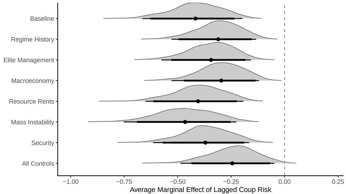
Figure D1. Average Marginal Effect of Coup Probability on Having Succession Rules with Correlated Random Effects
