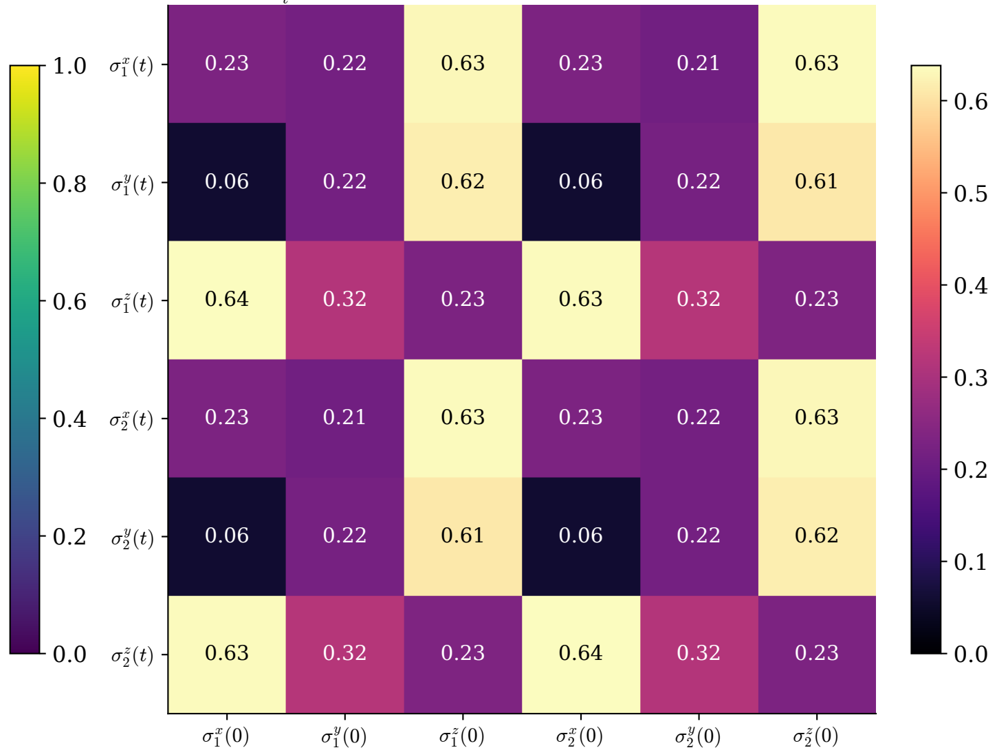
\max_t |C_{\text{esatto}}(t) - C_{\text{VQE}}(t)| (PMA base, \mathcal{F}=0.940 )
