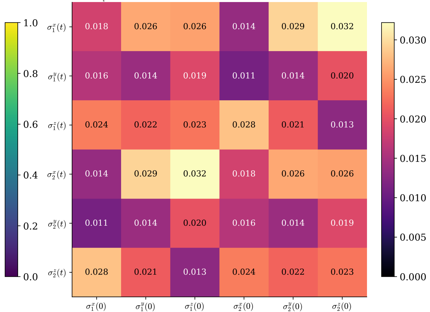
\max_t |C_{\text{esatto}}(t) - C_{\text{circuito}}(t)| (PMA esteso, \mathcal{F} = 1.000000 )
