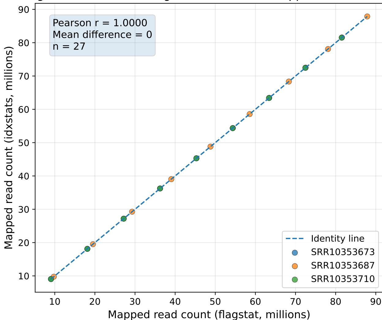
Agreement between flagstat and idxstats mapped-read counts
