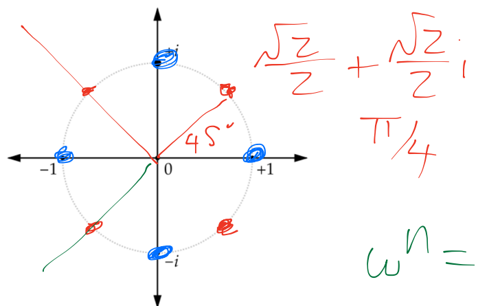
Figure 1: The complex roots of unity equally spaced around the unit circle.
