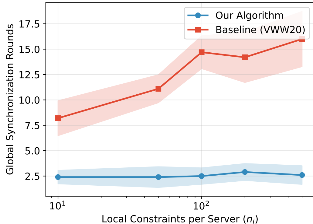
Exp A: Decoupling n from Sync Rounds
