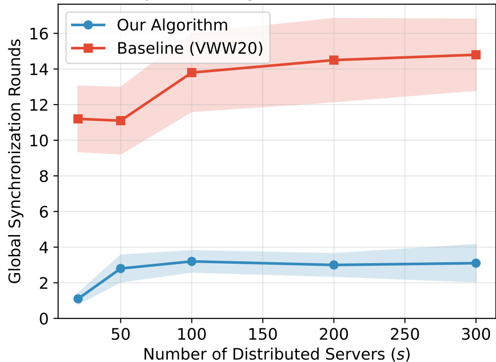
Exp B: Scaling with Network Size
