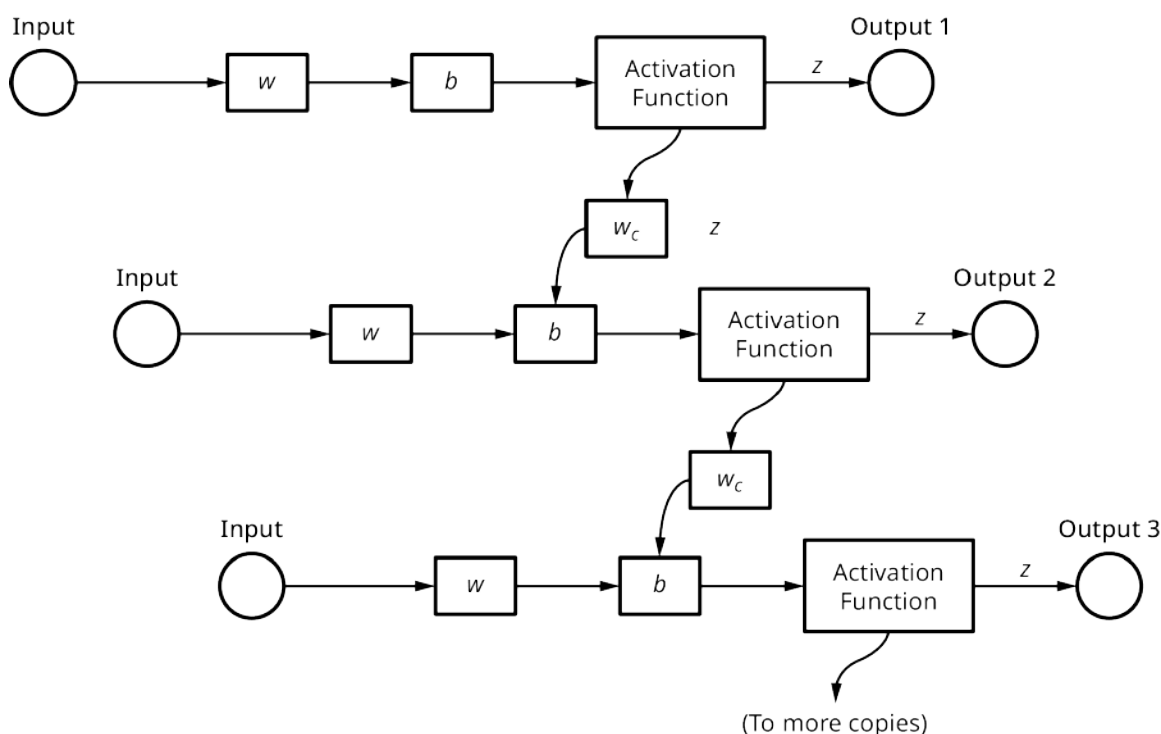
Figure 7.10 Unrolling an RNN
