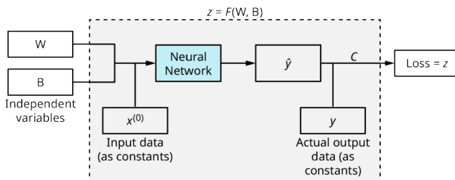
Figure 7.7 Neural Network with Loss Function C , Regarded as a Function of Weights and Biases. Given a set of weights \mathbf{W} and biases \mathbf{B} , the neural network is run on a set of input data \mathbf{x}^{(0)} , the output \hat{y} is obtained and compared against the actual output y via a loss function, C , providing a single number: the loss, z . The goal of training is to adjust \mathbf{W} and \mathbf{B} such that z is minimized.
