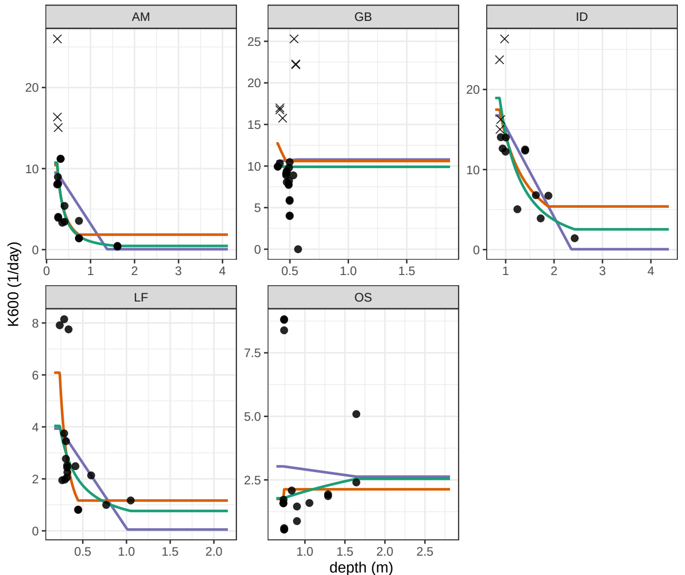
K600 rating curves on depth -- UNTRIMMED calibration data curves fit to ALL points; shape marks what trim_k600(EXCL='base') would drop
