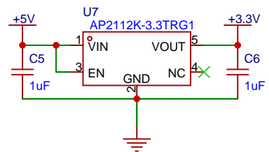
LDO-3.3V
