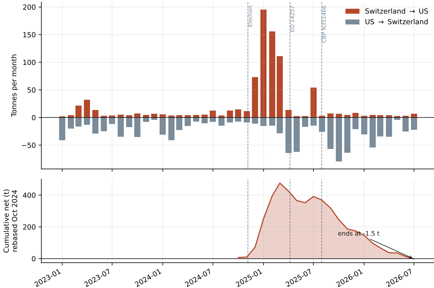
The round trip: Swiss--US gold flows, and their cumulative net
