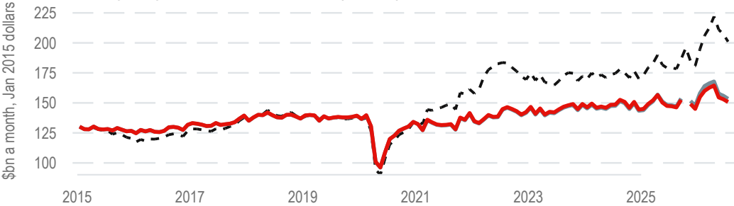
d. US goods exports: nominal, real, and real on the reweighted deflator Shaded: reweighting cuts measured real exports by $2.7bn a month
