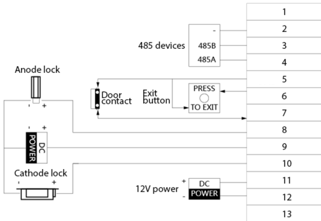
Figure 2-8 Cable connection
