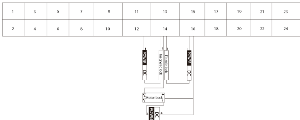
Figure 2-18 Lock cable connection
