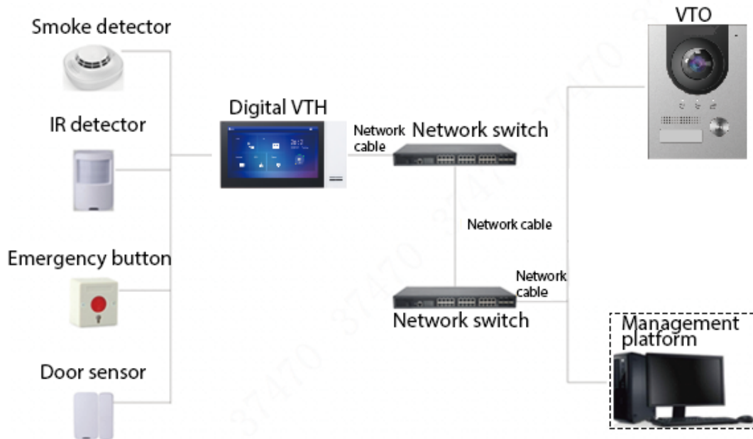
Figure 1-1 Network diagram
