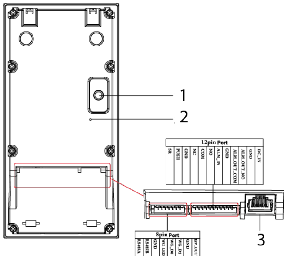
Figure 2-13 VTO3221E-P
