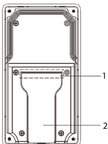
Figure 2-10 VTO3211D-P4
