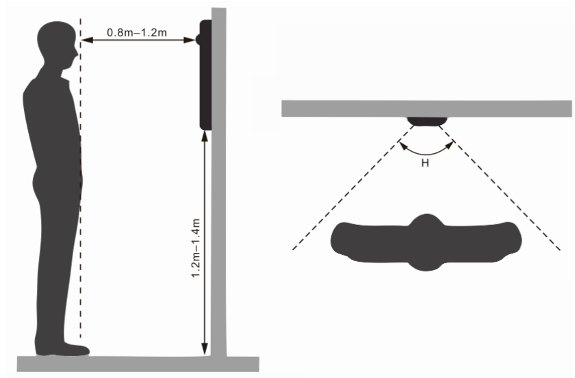
Figure 3-1 Installation position
