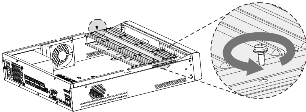
Figure 1-21 Remove screws (2U)
