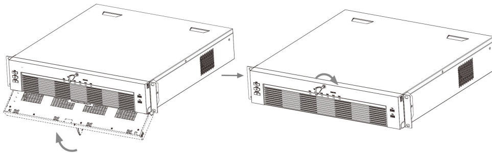
Figure 1-32 Lock front panel
