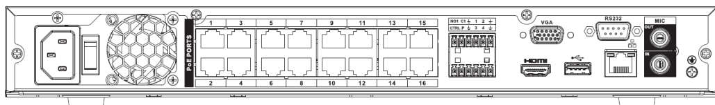
Figure 5-1 Rear panel of NVR2000 series
