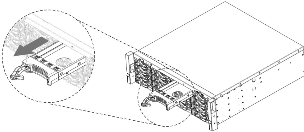
Figure 1-33 Take out HDD box
