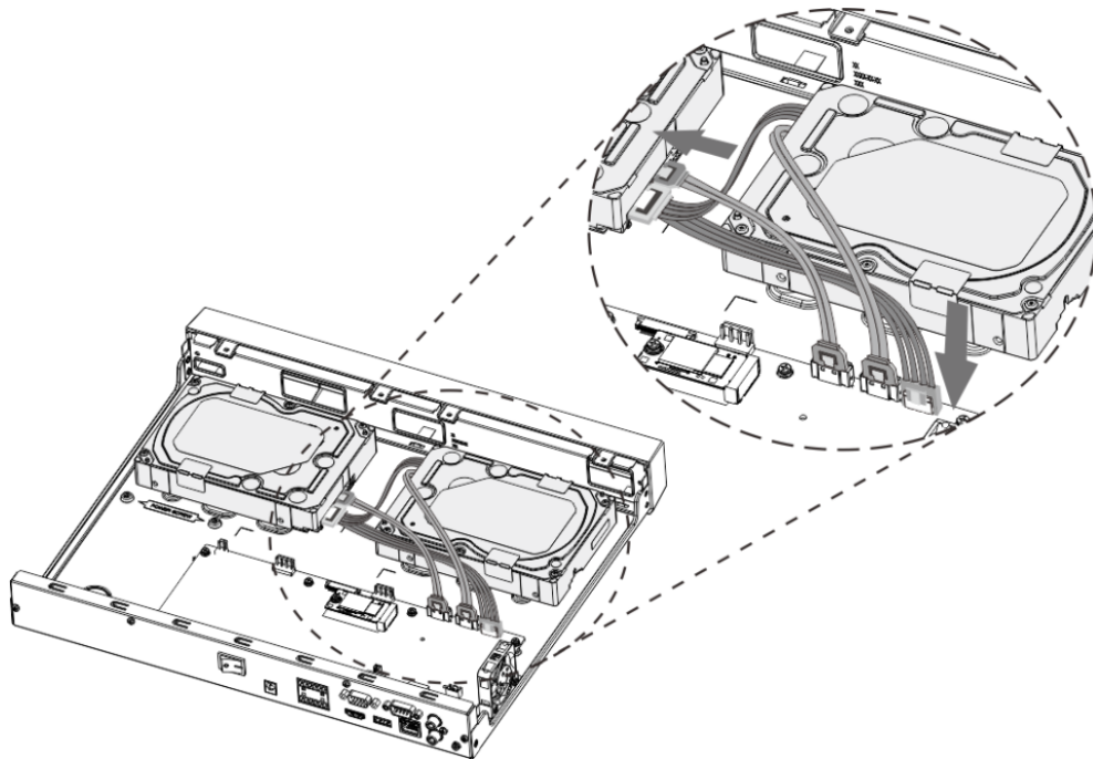
Figure 1-16 Connect cables
