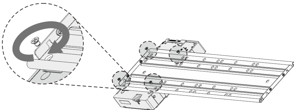
Figure 1-22 Fasten screws
