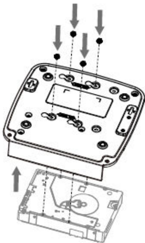
Figure 1-4 Secure screws
