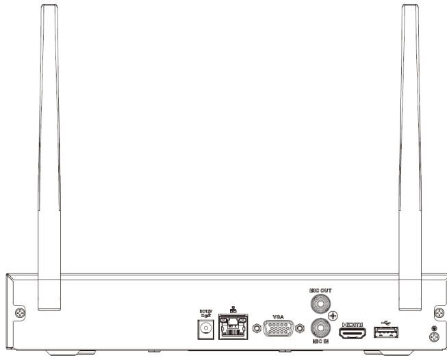
Figure 4-2 Rear panel of NVR1100-W-S2 series
