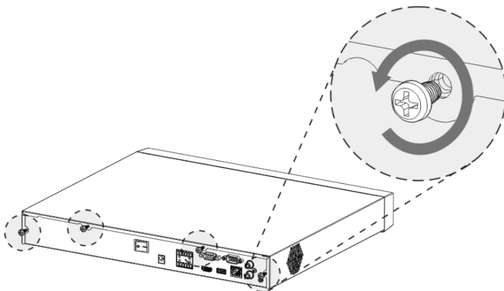
Figure 1-12 Remove screws
