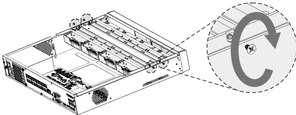
Figure 1-25 Fasten screws
