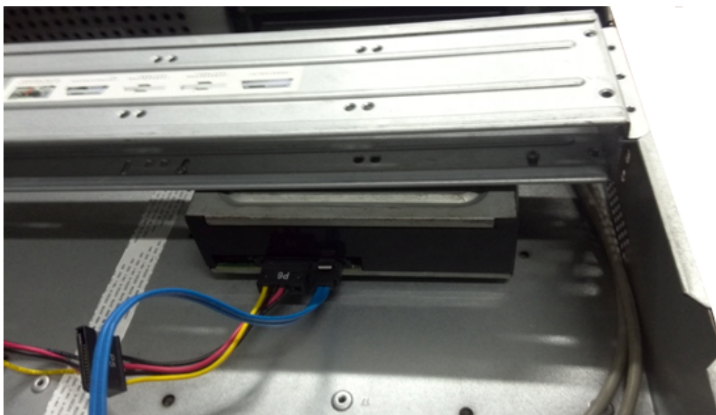
Figure 1-46 Connect cables
