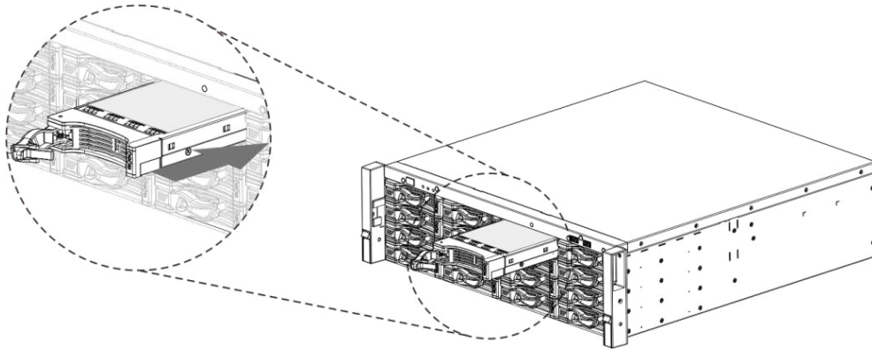
Figure 1-36 Close the handle
