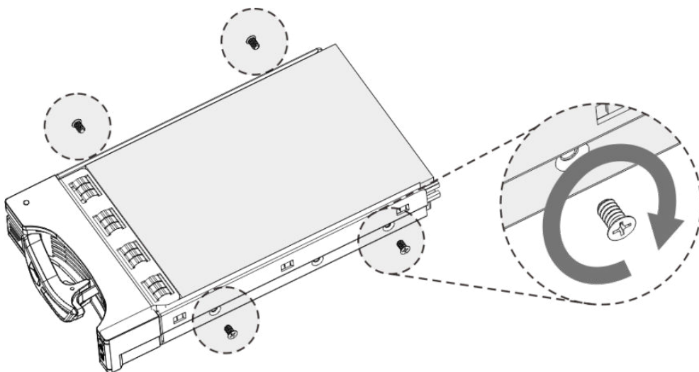
Figure 1-35 Fasten screws
