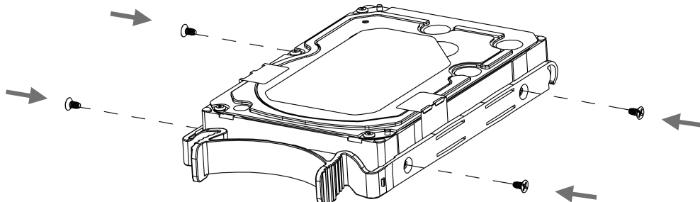
Figure 1-30 Fasten HDD
