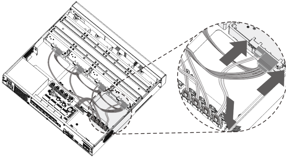
Figure 1-26 Connect cables
