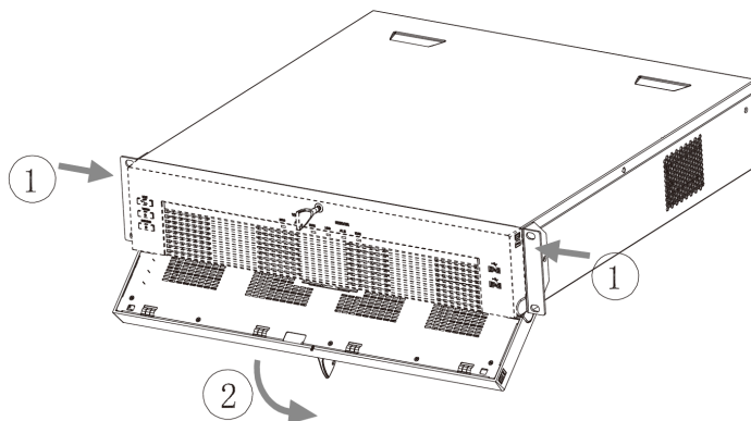
Figure 1-29 Open front panel
