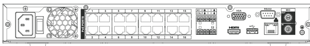
Figure 5-2 Rear panel of NVR4000 series
