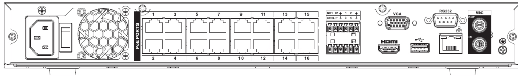
Figure 4-4 Rear panel of NVR2000-4KS3 series
