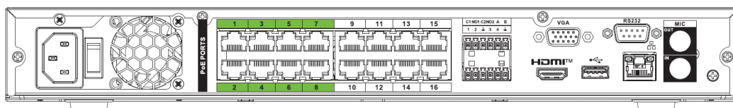
Figure 5-3 Rear panel of NVR5000 series
