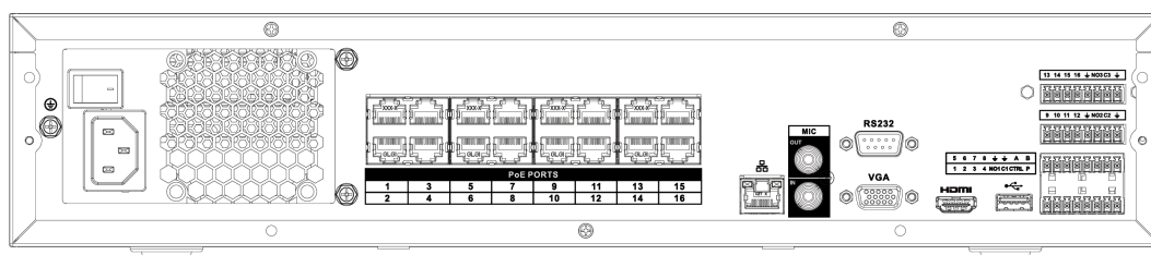
Figure 7-1 Rear panel of NVR4000 series
