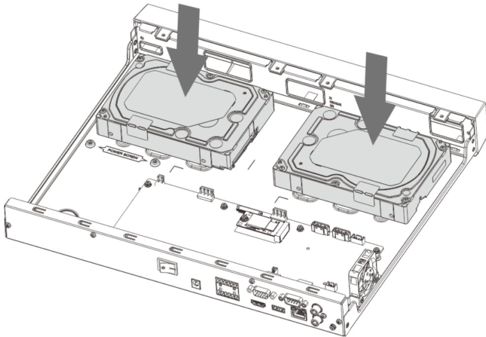
Figure 1-14 Align HDD
