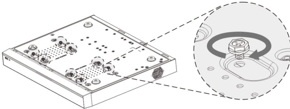
Figure 1-15 Fasten screws
