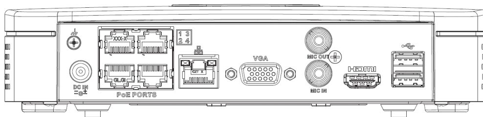
Figure 4-5 Rear panel of NVR2100-S3 series
