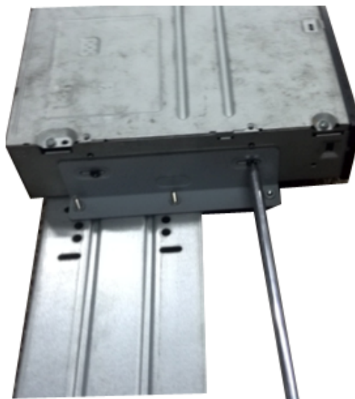
Figure 1-44 Fasten screws
