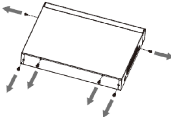
Figure 1-7 Loosen screws
