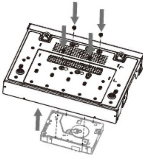
Figure 1-9 Align HDD
