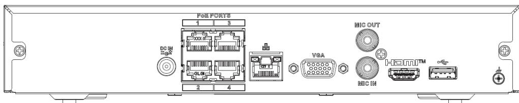
Figure 4-1 Rear panel of NVR1000-S3/H series
