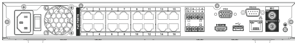
Figure 4-6 Rear panel of NVR4000 series
