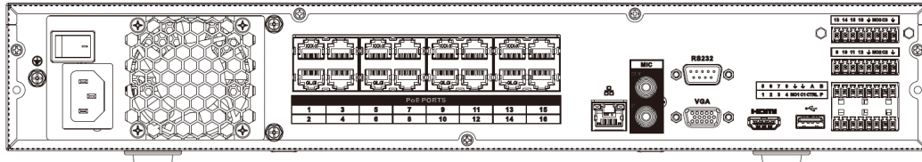
Figure 6-1 Rear panel of NVR4000 series
