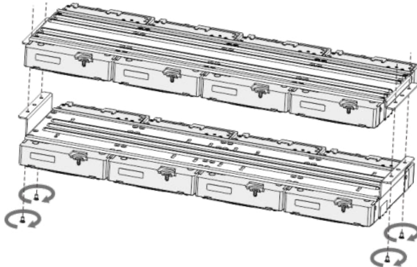
Figure 1-24 Lock brackets
