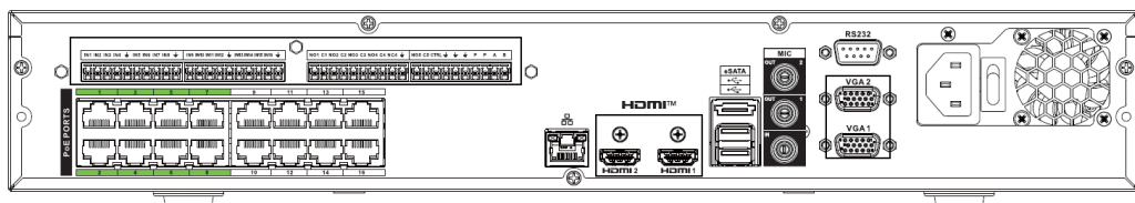
Figure 6-2 Rear panel of NVR5000 series
