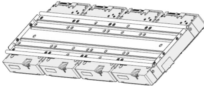
Figure 1-23 Install more HDDs
