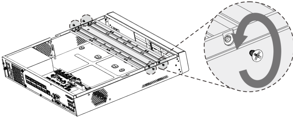
Figure 1-21 Remove screws (2U)
