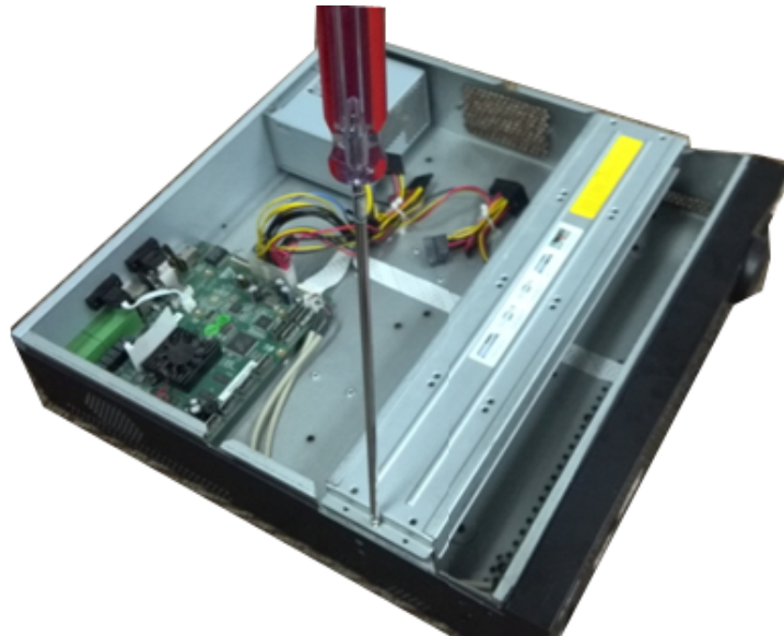
Figure 1-37 Open the top cover
