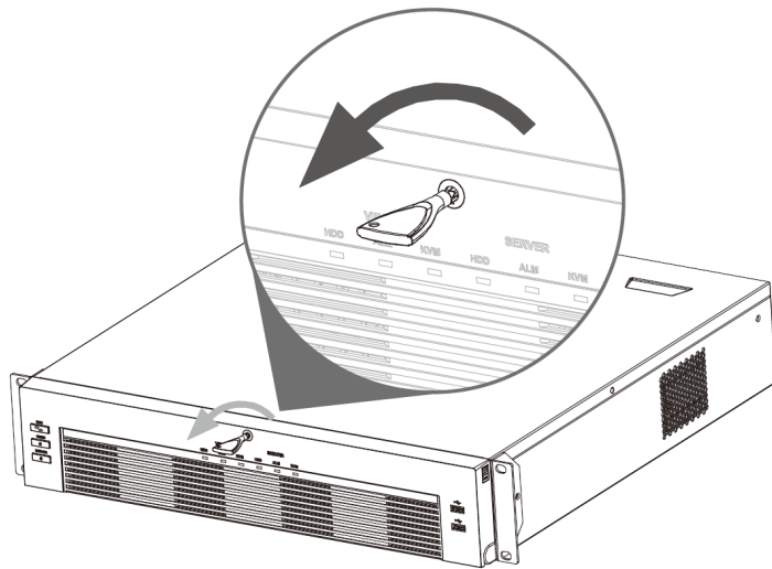
Figure 1-28 Unlock front panel
