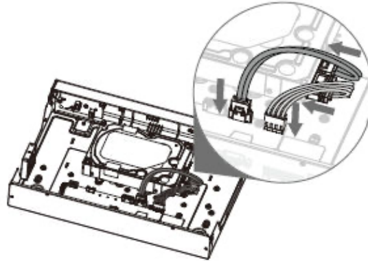
Figure 1-10 Connect cables
