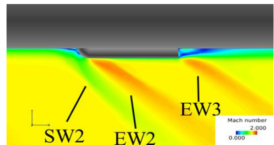
(b) Surroundings of protuberance.
