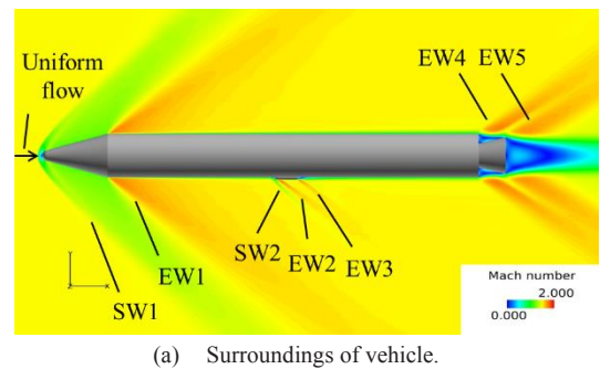
(a) Surroundings of vehicle.
