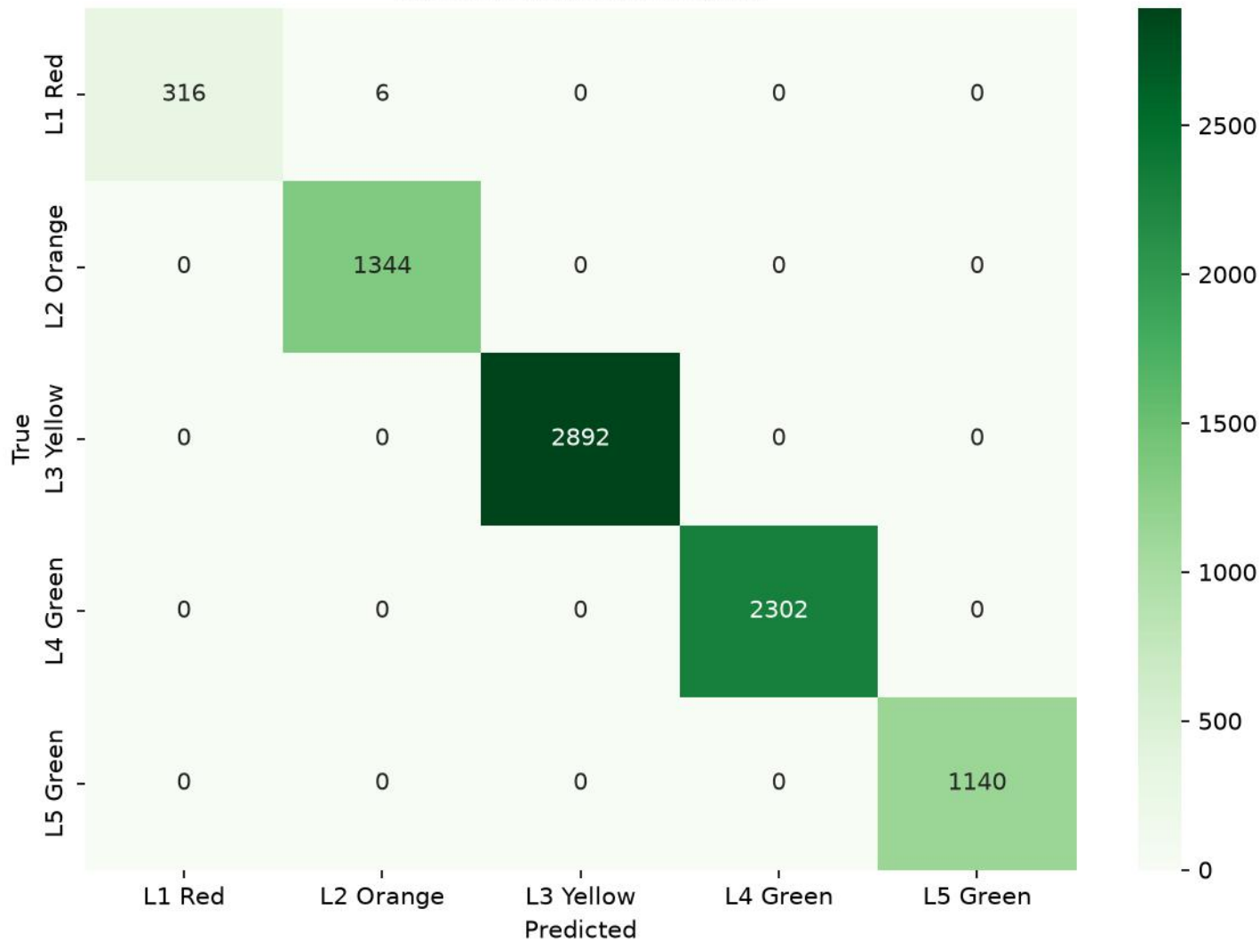
Baseline confusion matrix
