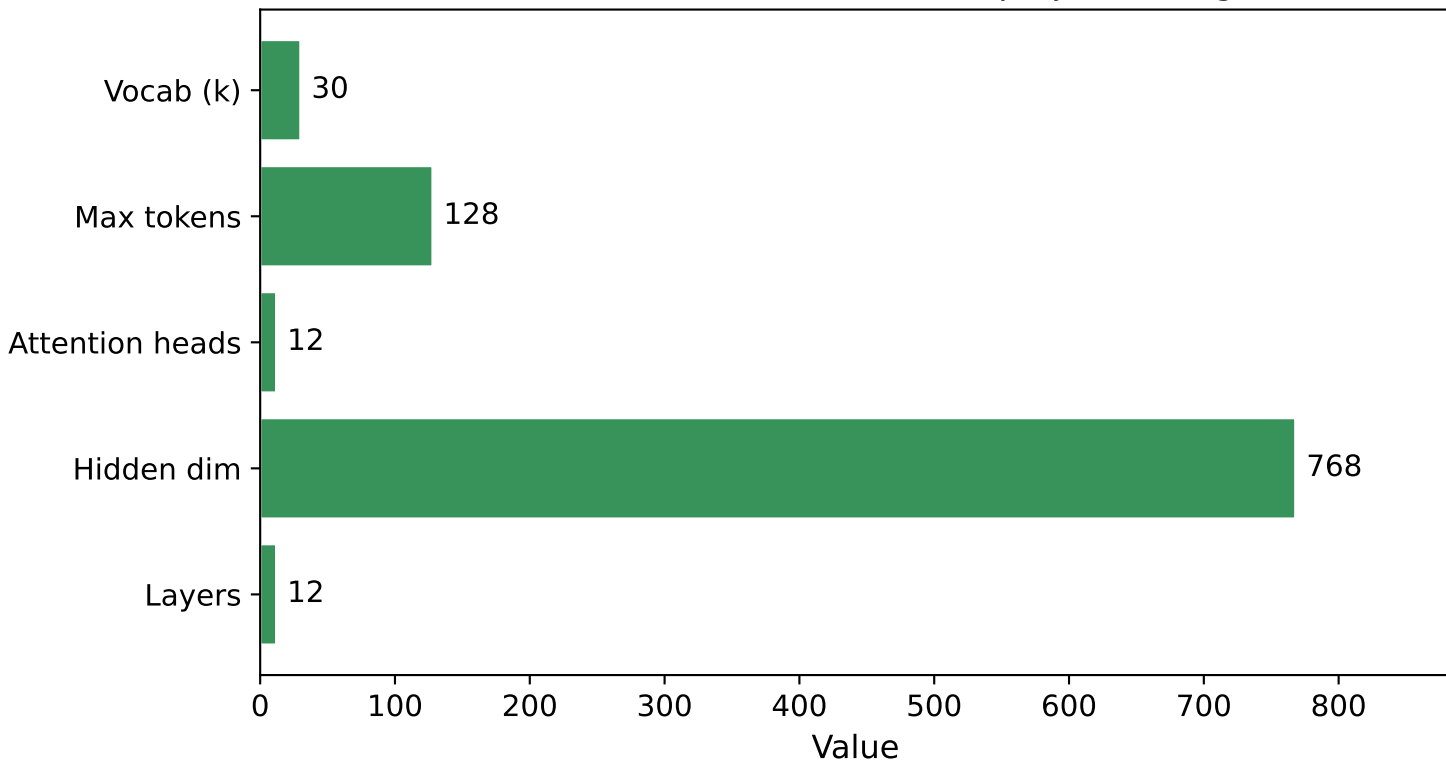
BioBERT-base architecture constants (project configuration)
