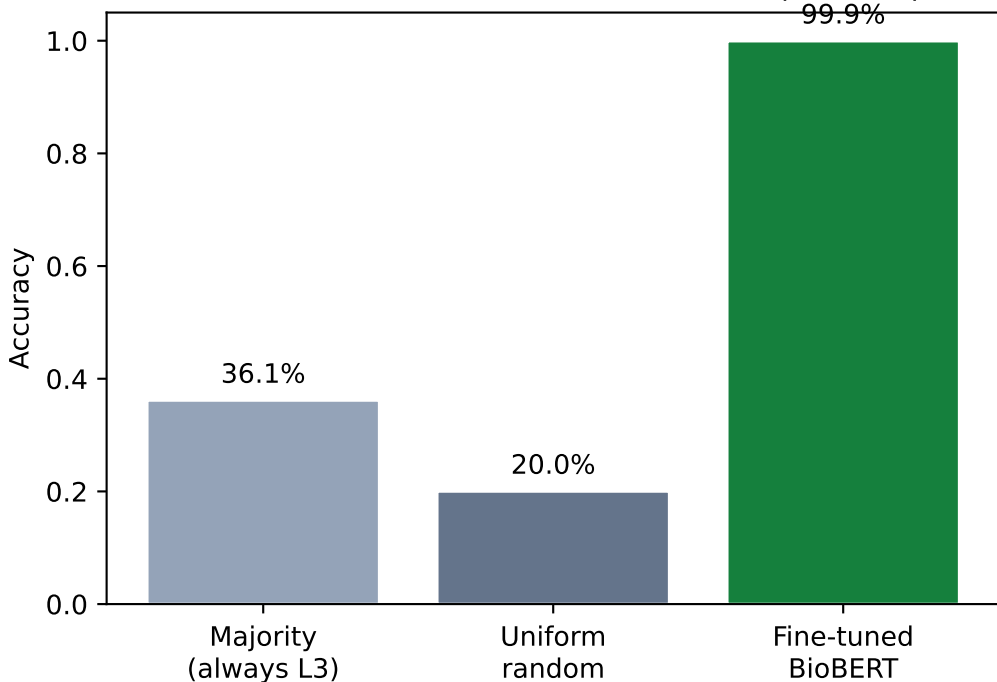
Naive baselines vs fine-tuned model (holdout)
