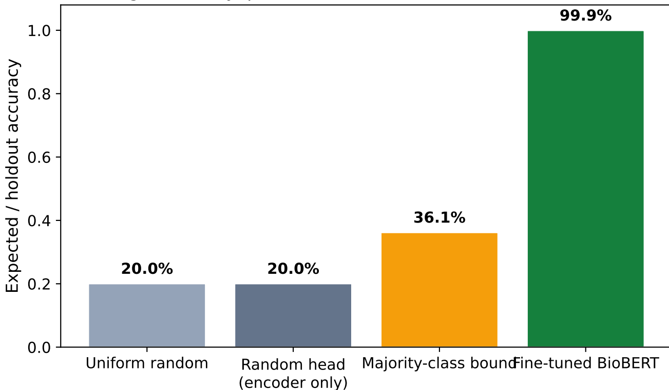
Triage accuracy: pre-fine-tune bounds vs fine-tuned BioBERT
