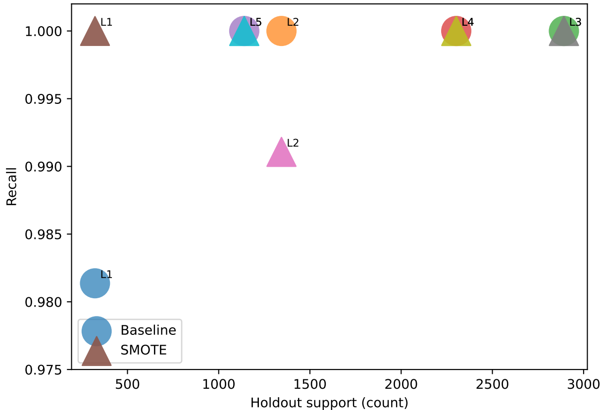
Recall vs class support (bubble size \propto F1)
