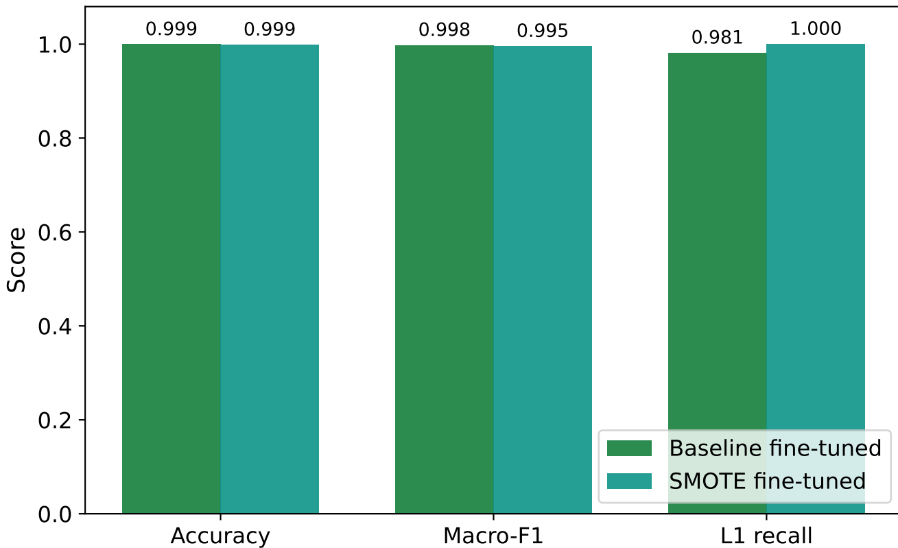
Headline holdout metrics: baseline vs SMOTE
