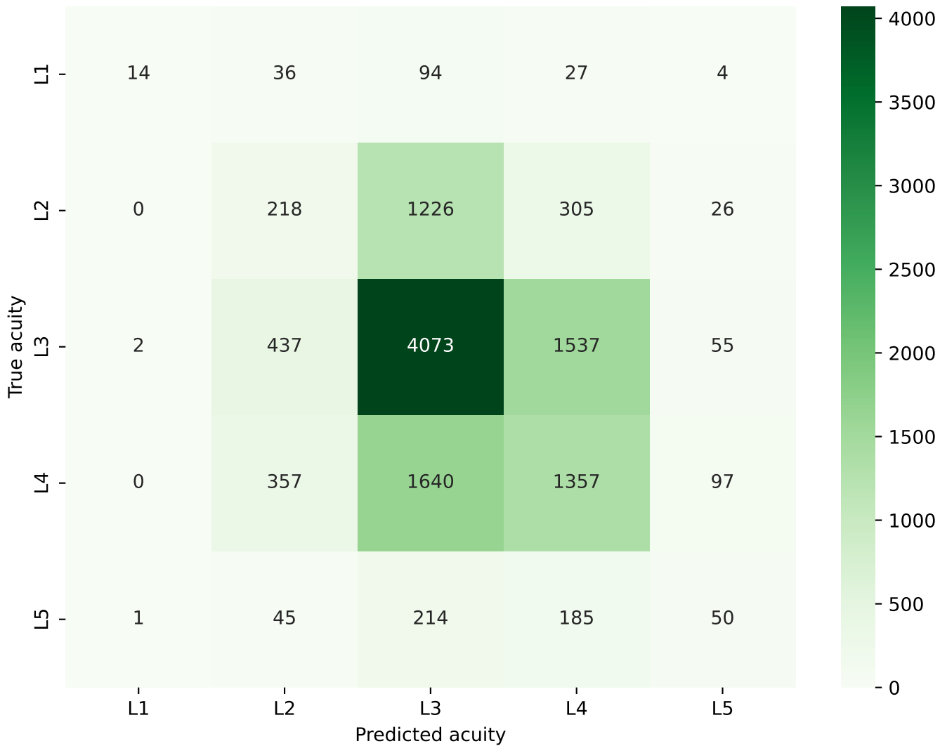
Baseline — nhamcs
