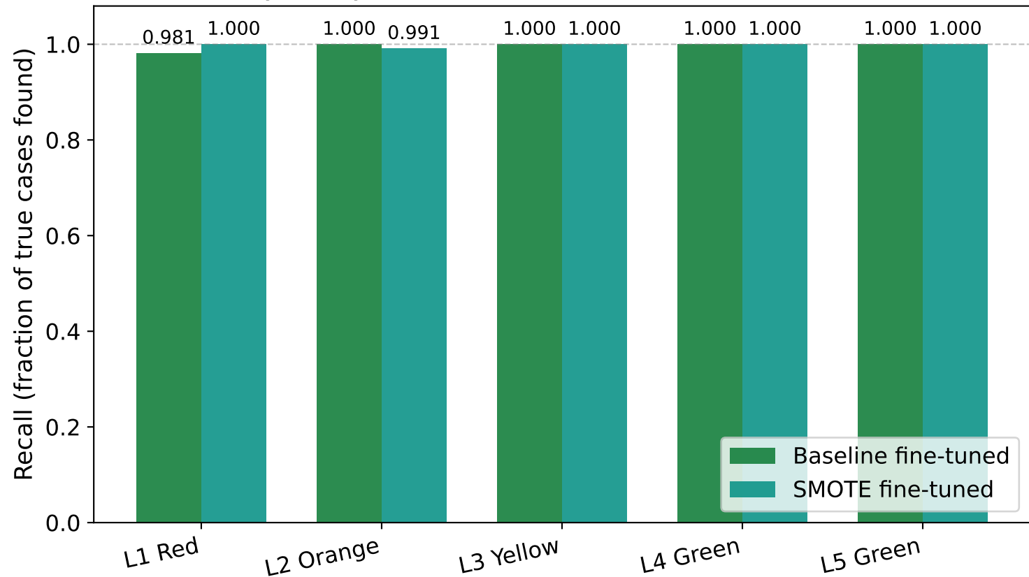
Recall by acuity level: baseline vs SMOTE (holdout, N=8,000)
