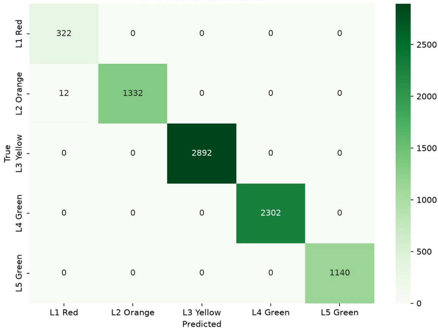
SMOTE confusion matrix
