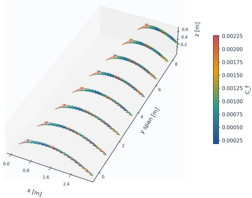
Fig. 42. Upper-surface flow direction coloured by C_f (chordwise only — the strip formulation carries no span-wise wall shear).
