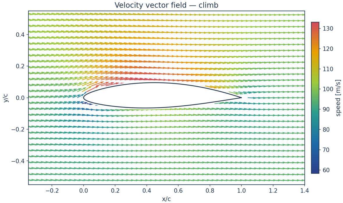
Fig. 35. Velocity vector field — climb.
