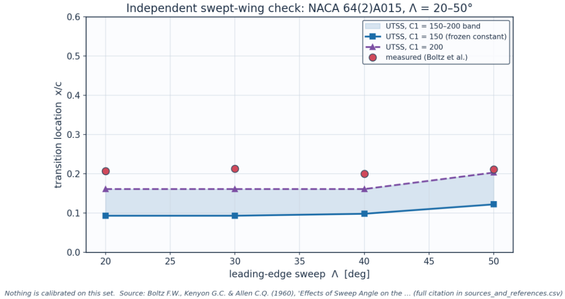
Fig. 52. Transition location against sweep angle, NACA 64(2)A015, with the C1 = 150-200 band shaded.
