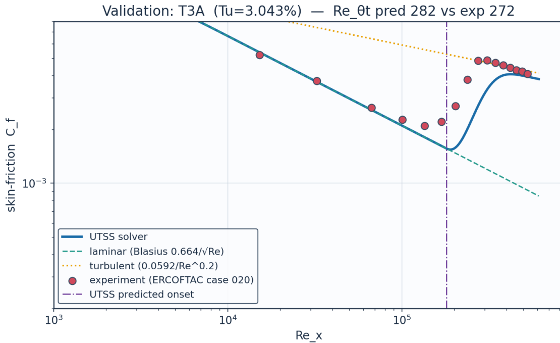
Fig. 40. Validation — ERCOFTAC T3A flat plate ( Tu = 3.0\% , bypass).
