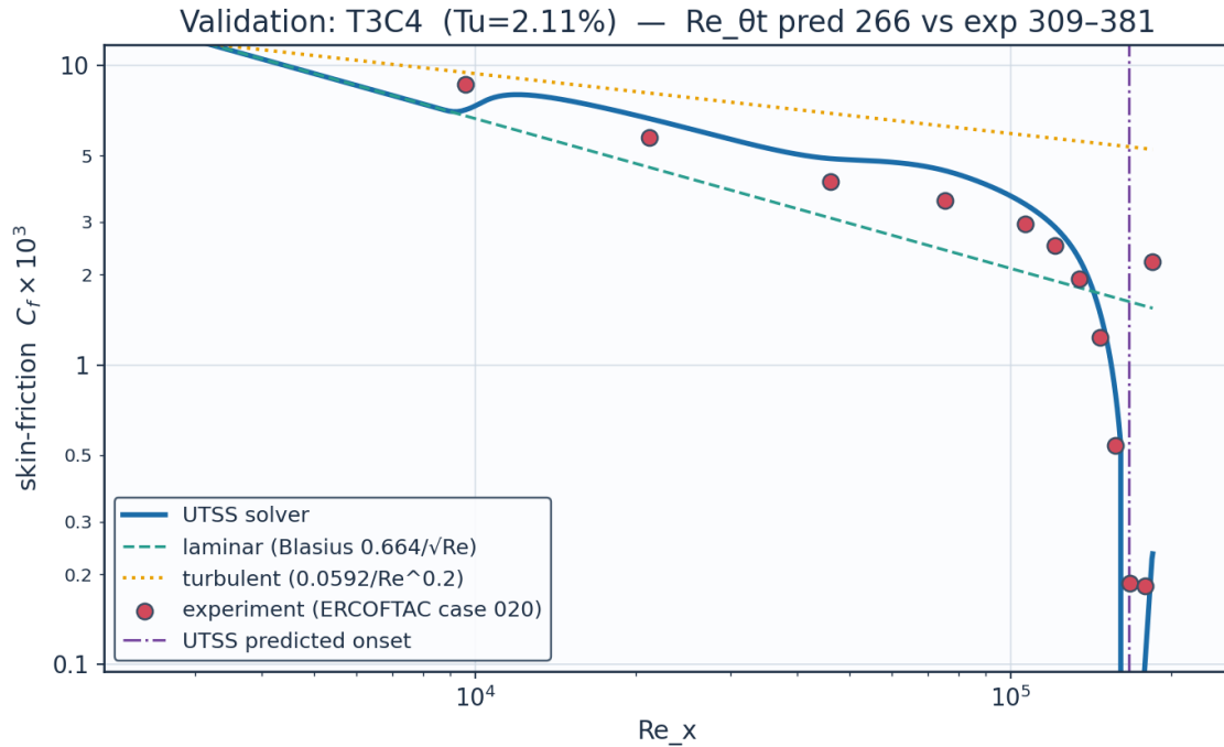
Fig. 46. Validation — ERCOTAC T3C4 flat plate (laminar separation bubble).
