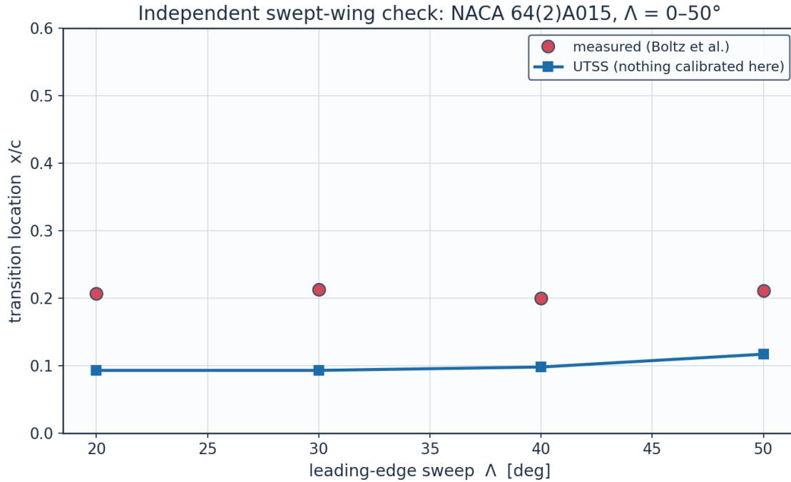
Fig. 43. Transition location against sweep angle, NACA 64(2)A015.
