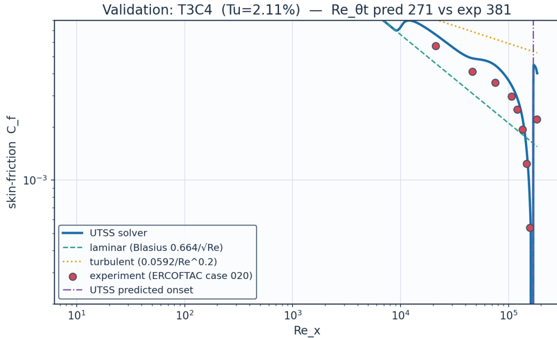
Fig. 38. Validation — ERCOFTAC T3C4 flat plate (laminar separation bubble).
