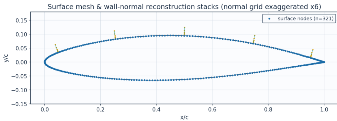
Fig. 9. Surface mesh and wall-normal stacks.
