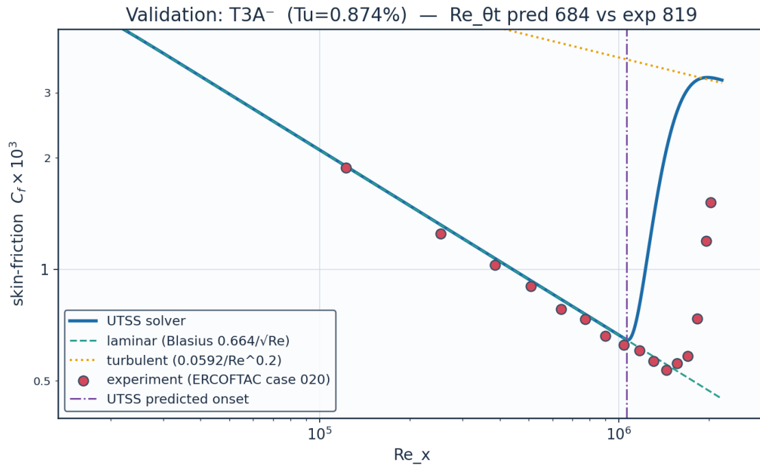
Fig. 44. Validation — ERCOFTAC T3A - flat plate (Tu = 0.87 %, bypass).
