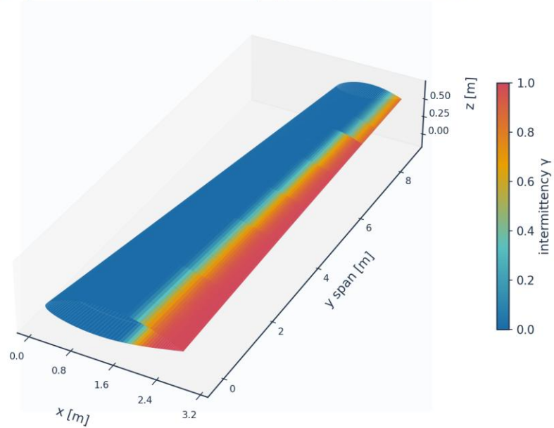
Fig. 41. 3-D wing surface contour — intermittency \gamma (transition front).
