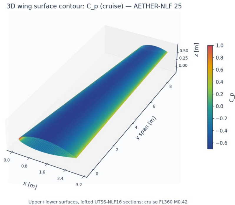
Fig. 39. 3-D wing surface contour — pressure C_p .
