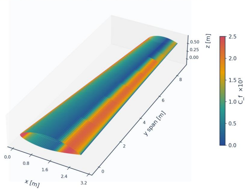
Fig. 40. 3-D wing surface contour — skin friction C_f (\times 10^3) .
