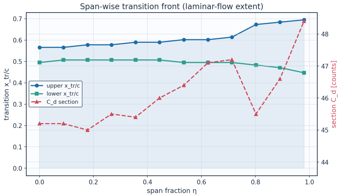
Fig. 29. Span-wise transition front and section drag.
