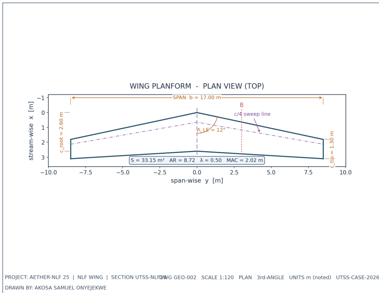
Fig. 2. Wing planform — plan (top) view, dimensioned.
