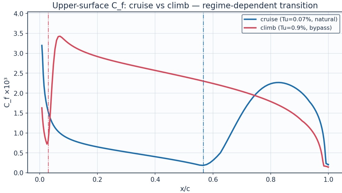
Fig. 26. C_f cruise vs climb — regime-dependent transition.
