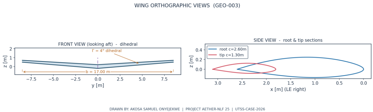
Fig. 5. Front and side orthographic views.
