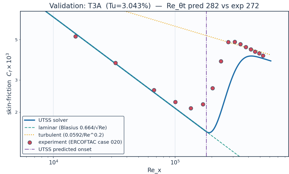
Fig. 43. Validation — ERCOFTAC T3A flat plate ( Tu = 3.0\% , bypass).
