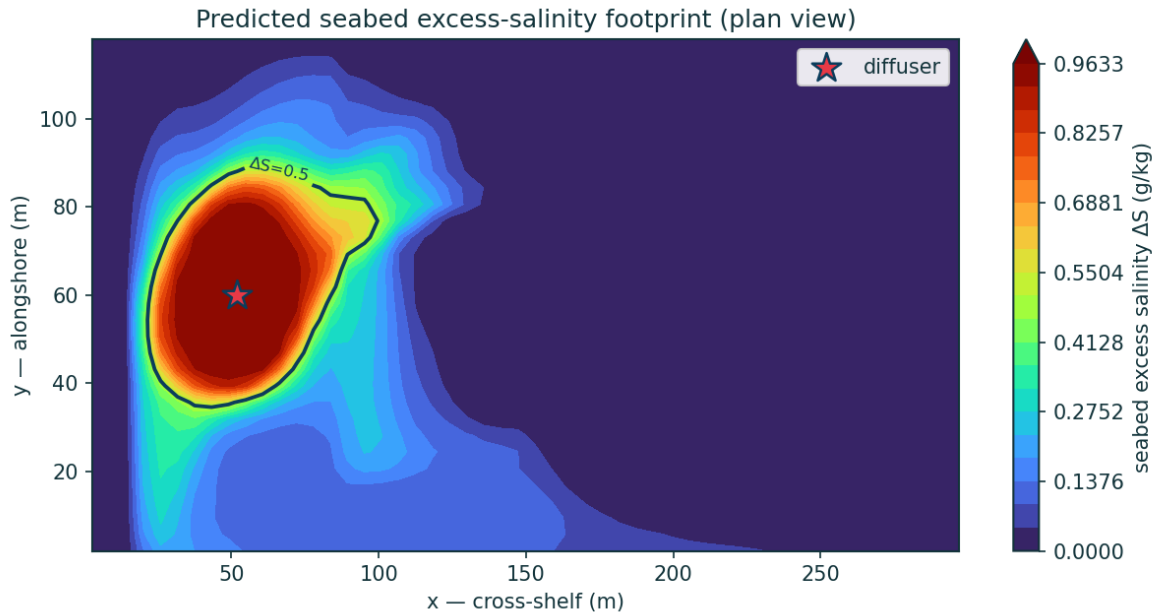
Figure 1 — Predicted seabed excess-salinity footprint (plan view), with the \Delta S_{crit} assessment contour.
