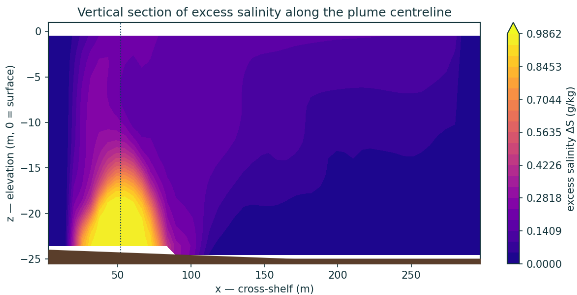
Figure 3 — Vertical section of excess salinity along the plume centreline, showing the bottom-trapped dense gravity-current layer (§12.4).
