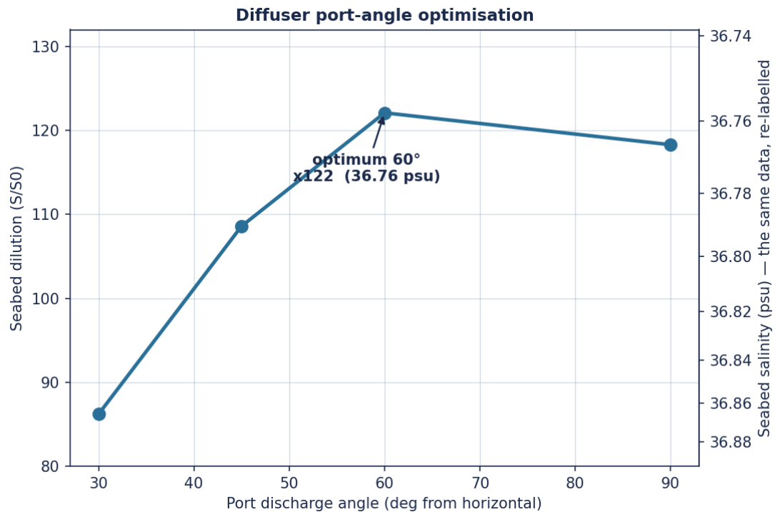
Figure. Diffuser port-angle optimisation: seabed dilution vs port discharge angle. The right-hand axis re-labels the same curve as seabed salinity, which is a fixed function of dilution, not an independent measurement.
