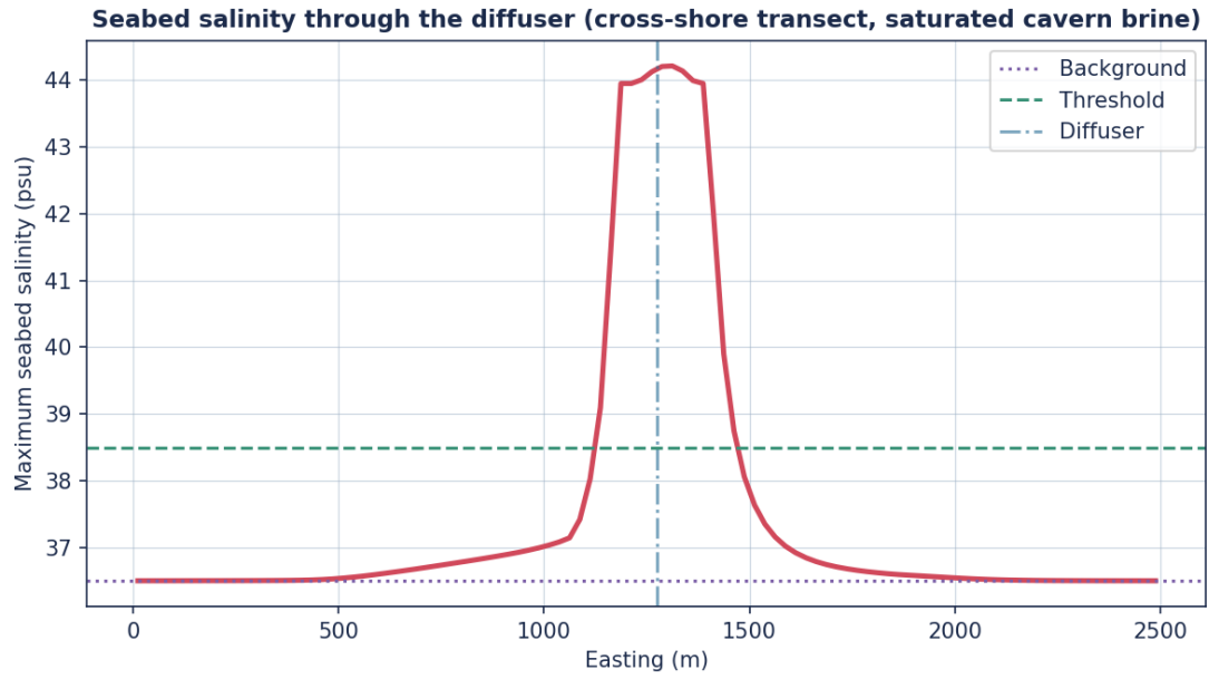
Figure. Maximum seabed salinity along a transect through the diffuser (neap, full flow, saturated cavern brine).
