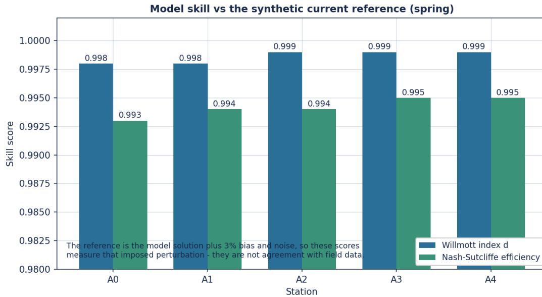
Figure. Index-of-agreement between the model and the synthetic current reference by station (spring). The reference is derived from the model solution, so this is not a field comparison.
