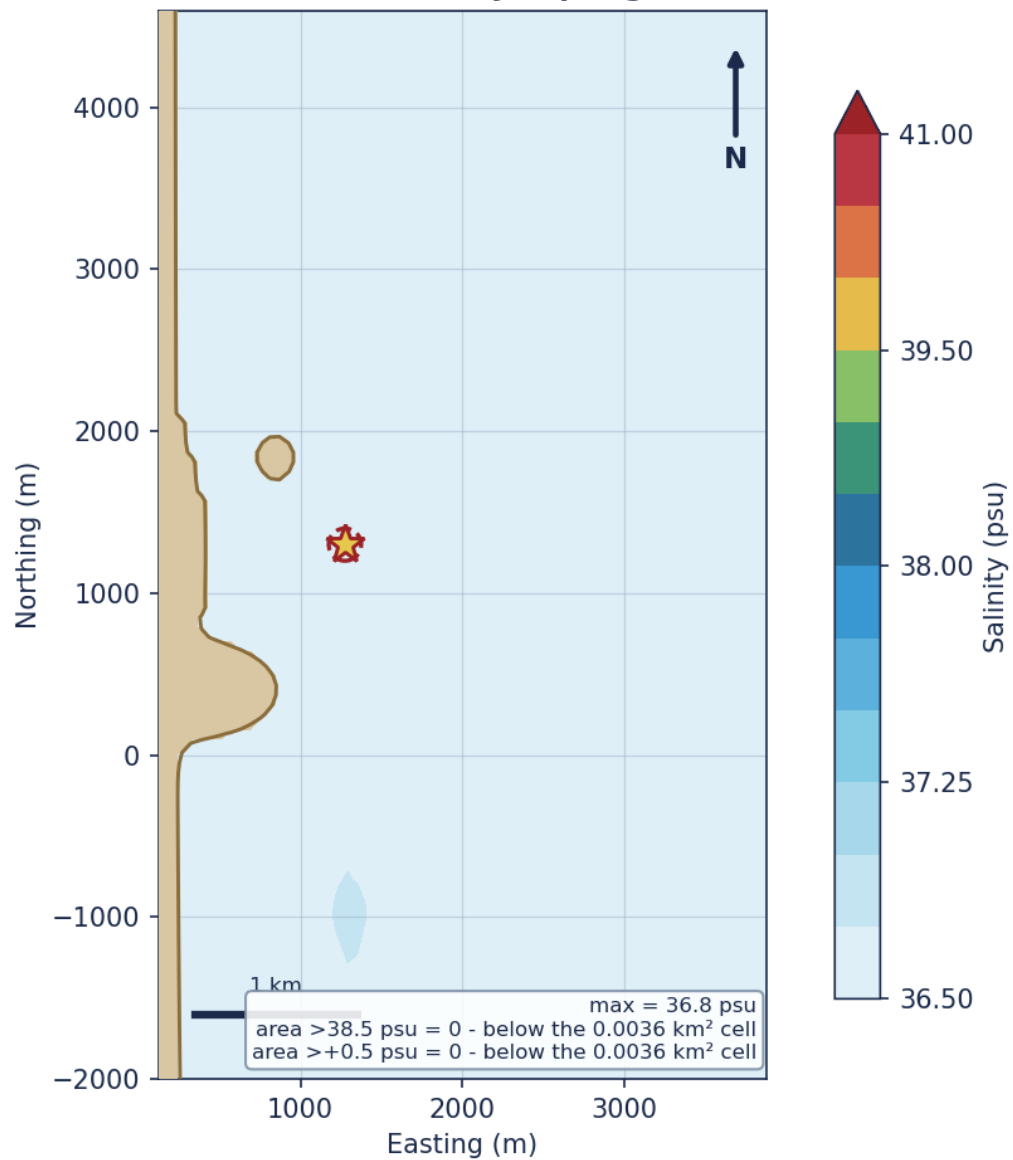
Figure. Far-field maximum seabed salinity - spring, full flow (RO brine)
