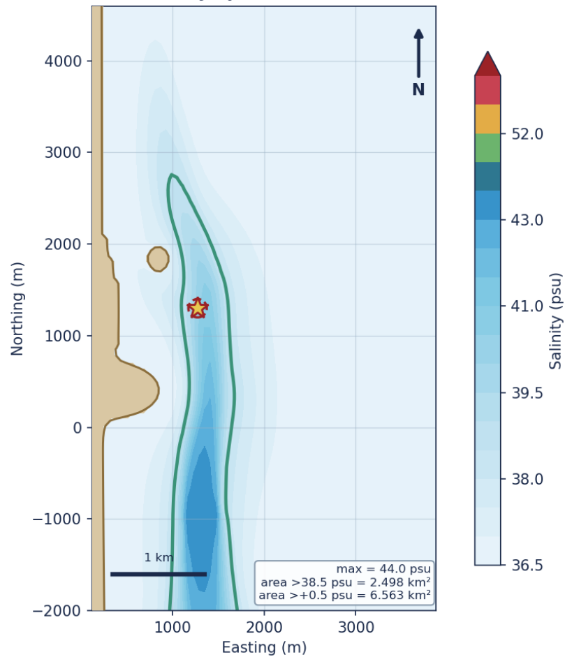
Figure. Far-field maximum seabed salinity - phase-2 saturated cavern brine (worst case)
