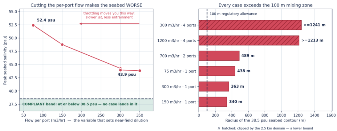
Figure. Phase-2 cavern brine: peak seabed salinity and 38.5 psu mixing-zone radius against discharge flow and port count. Every case exceeds the threshold, and reducing the per-port flow makes the peak worse because near-field dilution is driven by exit momentum. The constraint is dilution, not load: a 250 psu source needs ~107:1 to reach 38.5 psu and the diffuser delivers 14-50:1.
