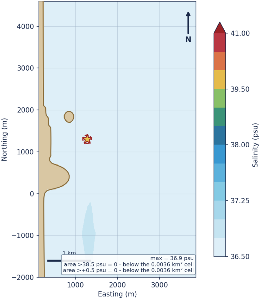
Far-field maximum seabed salinity - spring-neap envelope (full flow, RO brine)
