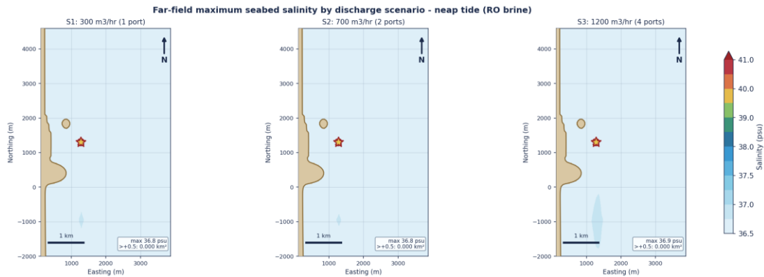
Figure. Far-field maximum seabed salinity by discharge scenario - neap tide (RO brine)
