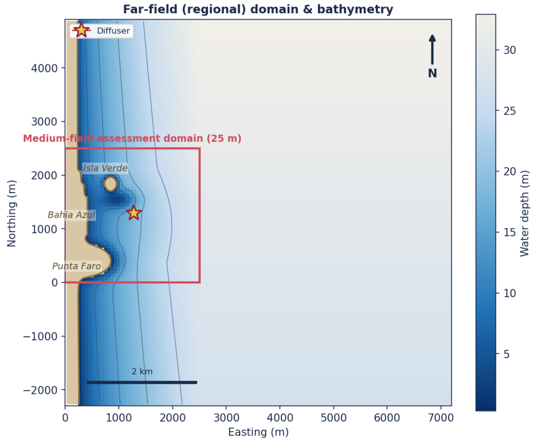
Figure. Far-field (regional) domain & bathymetry
