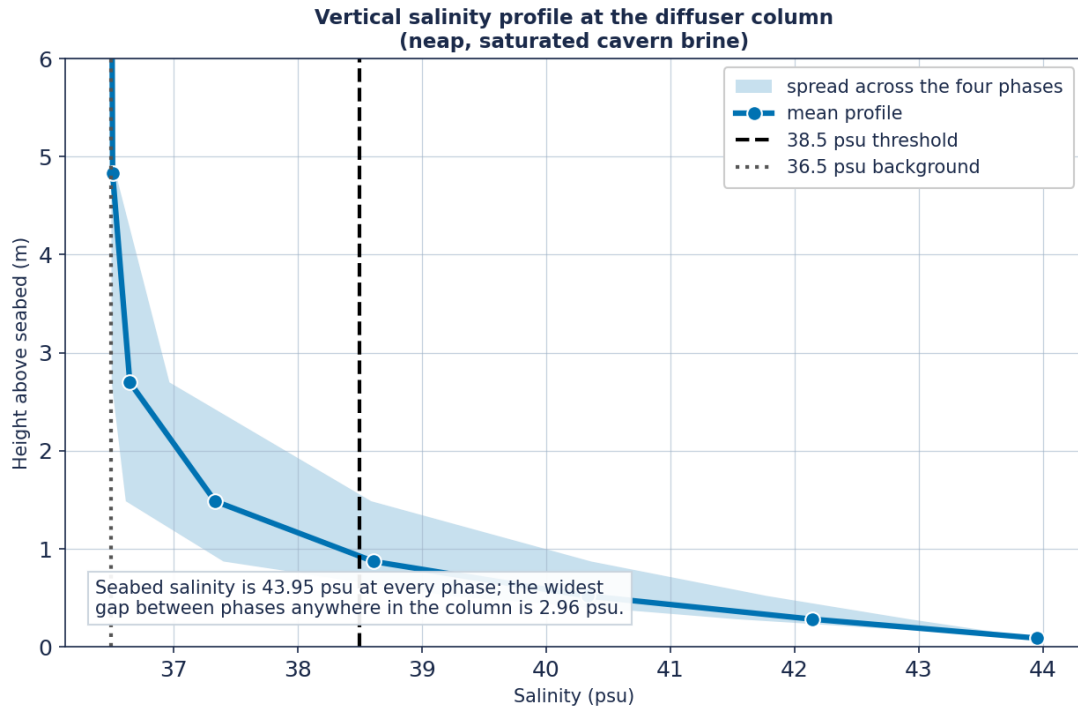
Figure. Vertical salinity profiles at the diffuser column - all tidal phases (neap, saturated cavern brine)
