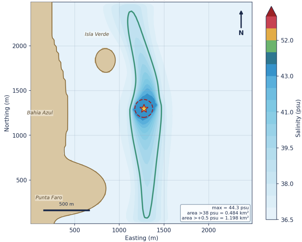
Maximum seabed salinity over a full spring-neap cycle (full flow, saturated cavern brine)
