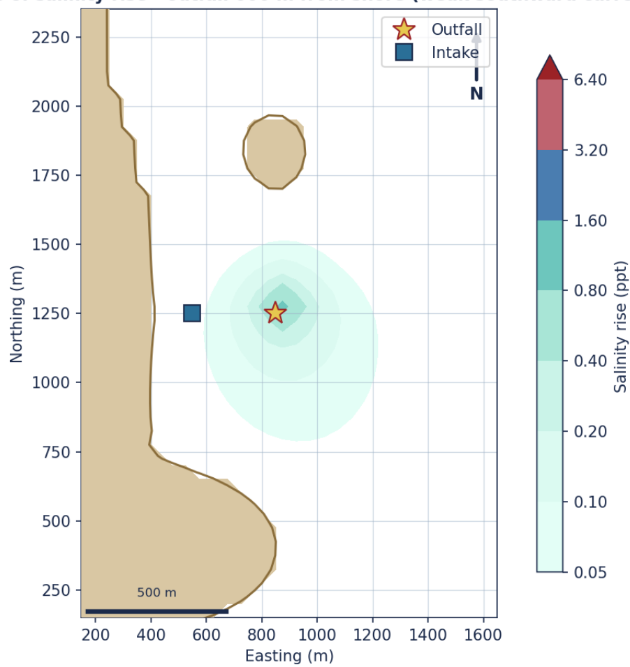
Figure. Salinity-rise contours, outfall 600 m from shore, weak southward current.
