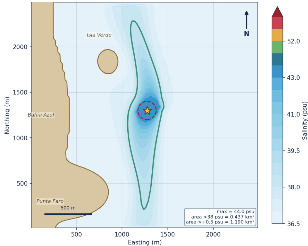
Maximum seabed salinity - 9-layer model (full flow, neap, saturated cavern brine)
