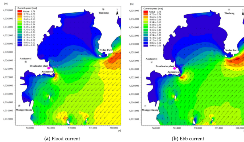
Figure 7. Hydrodynamic flow field simulation results.
