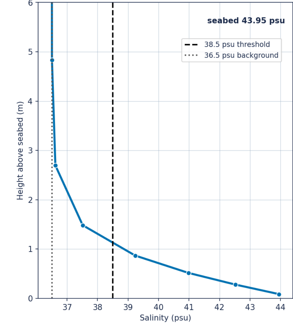
Vertical salinity profile at low water - neap (saturated cavern brine)
