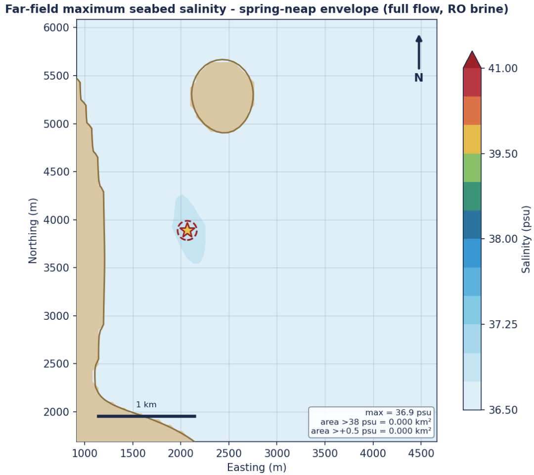
Figure. Far-field maximum seabed salinity - spring-neap envelope (full flow, RO brine)
