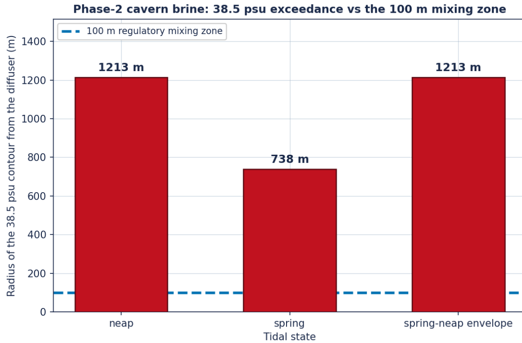
Figure. Phase-2 saturated cavern brine at full flow: the 38.5 psu seabed threshold is exceeded out to 1213 m from the diffuser on the neap envelope, over 0.484 km 2 of seabed - far outside the 100 m regulatory mixing zone. The RO concentrate of phase 1 does not exceed the threshold anywhere.
