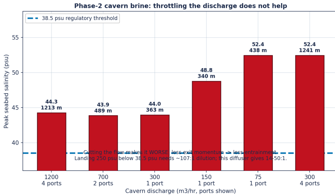
Figure. Phase-2 cavern brine: peak seabed salinity and 38.5 psu mixing-zone radius against discharge flow and port count. Every case exceeds the threshold, and reducing the per-port flow makes the peak worse because near-field
