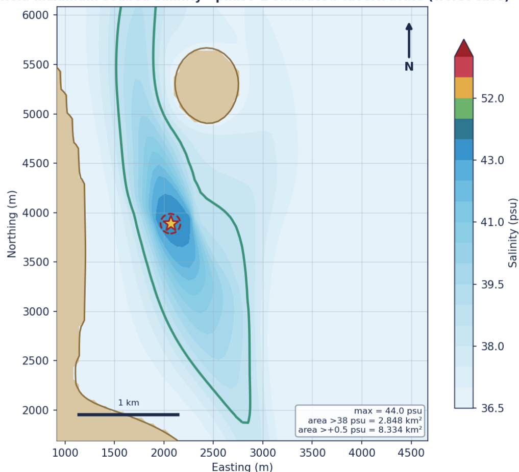
Figure. Far-field maximum seabed salinity - phase-2 saturated cavern brine (worst case)
