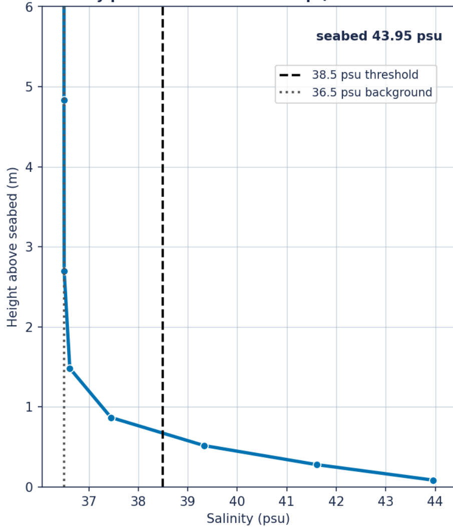
Figure. Vertical salinity profile at mid flood - neap (saturated cavern brine)
