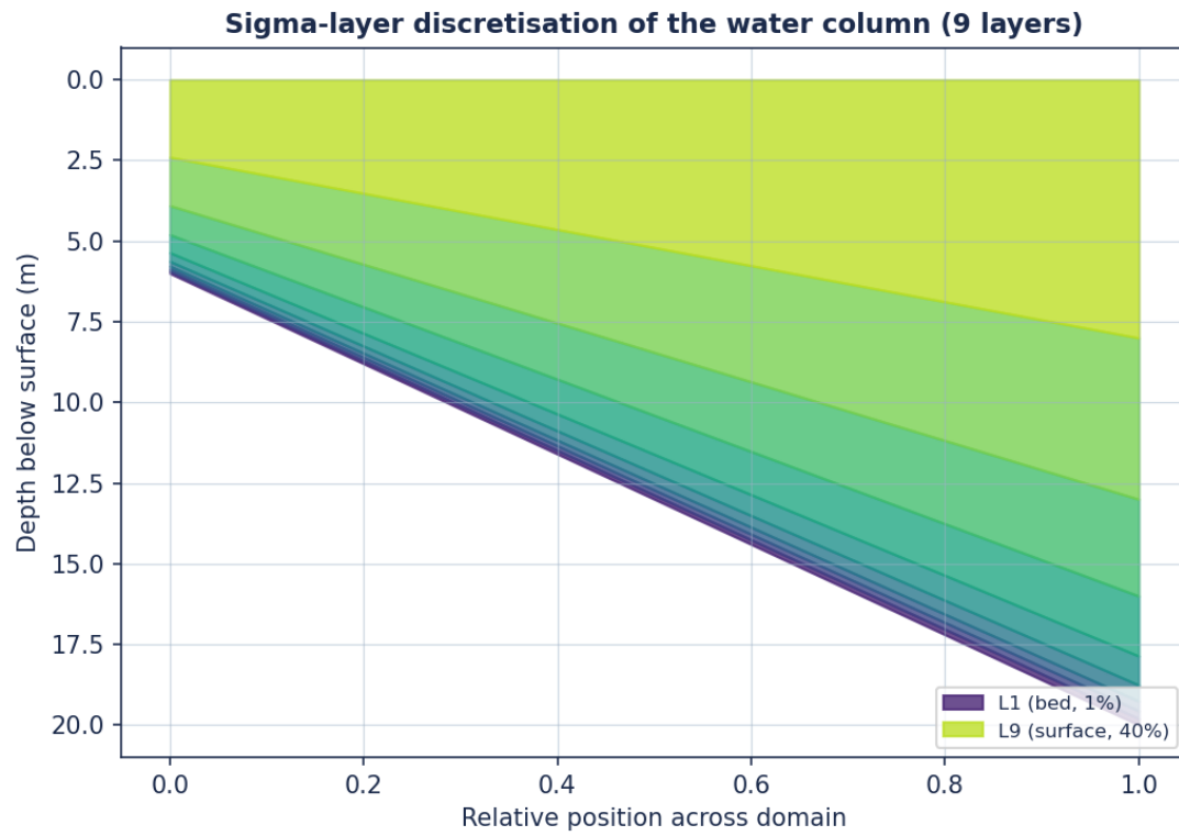
Figure. Terrain-following sigma layers versus water depth (9-layer scheme). Layers are numbered from the seabed upward, so L1 is the thin bed cell that resolves the dense bottom plume and L9 is the thick surface cell.
