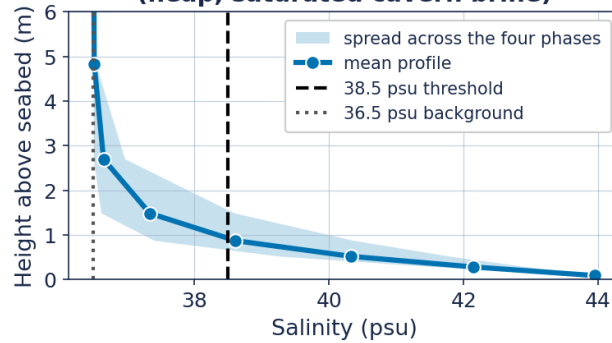
Figure. Vertical salinity profiles at the diffuser column - all tidal phases (neap, saturated cavern brine)
