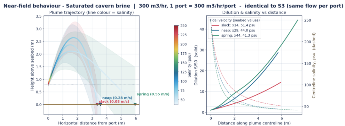
Figure. Near-field trajectory, dilution and salinity - Saturated cavern brine, 300 m 3 /hr (300 m 3 /hr per port).
