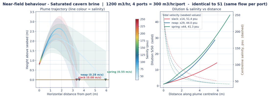
Figure. Near-field trajectory, dilution and salinity - Saturated cavern brine, 1200 m 3 /hr (300 m 3 /hr per port).
