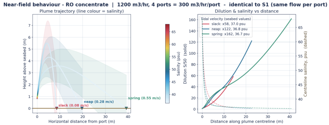
Figure. Near-field trajectory, dilution and salinity - RO concentrate, 1200 m 3 /hr (300 m 3 /hr per port).
