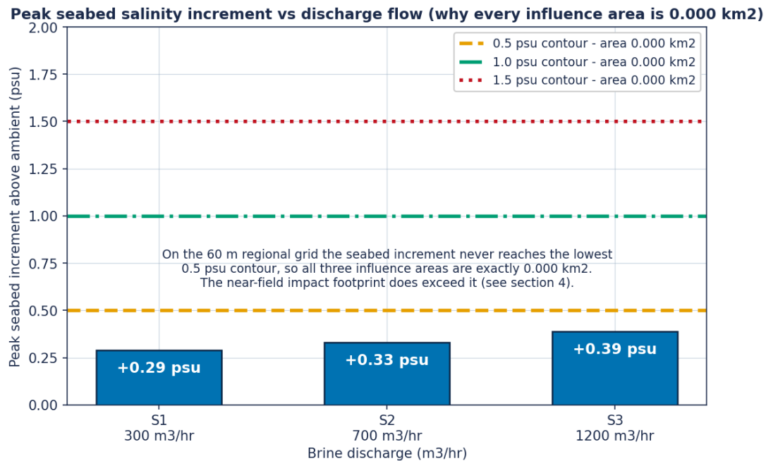
Figure. Peak seabed salinity increment by discharge scenario, against the 0.5, 1.0 and 1.5 psu contour thresholds. The increment peaks at 0.39 psu, so every influence area is 0.000 km 2 ; the zeros are grid-resolved, not absolute.
