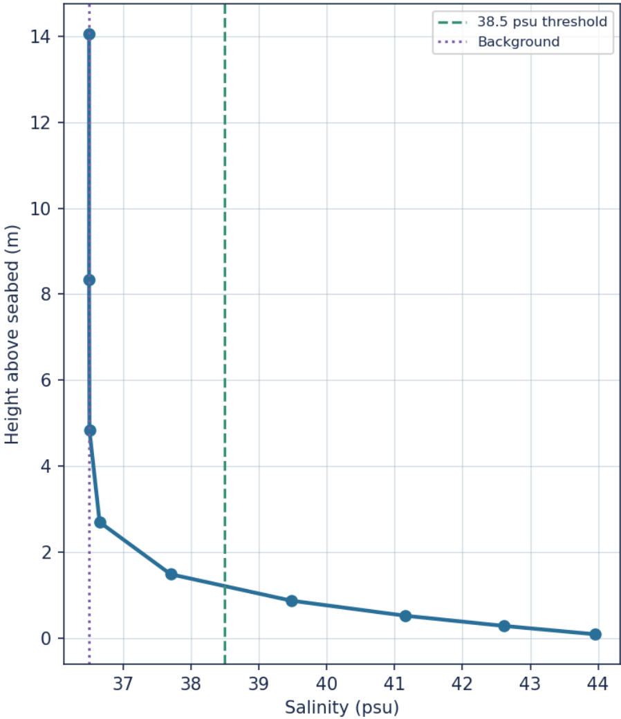
Vertical salinity profile at low water - neap (saturated cavern brine)
