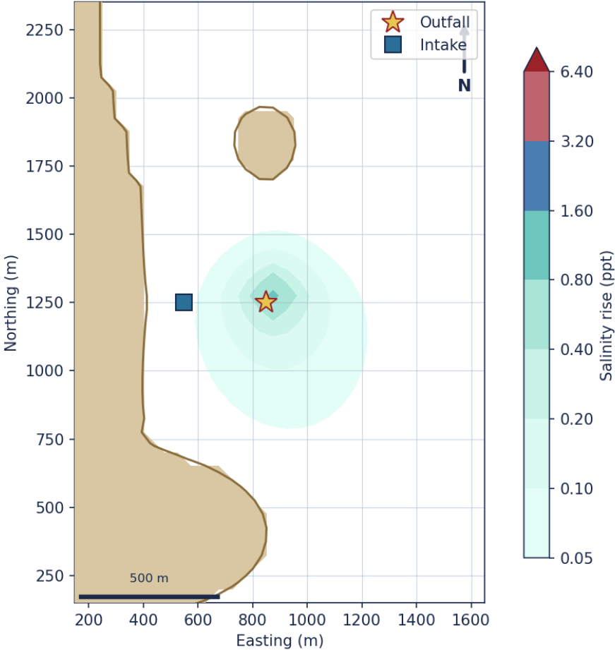
Contours of salinity rise - outfall 600 m from shore (weak southward, RO brine)
