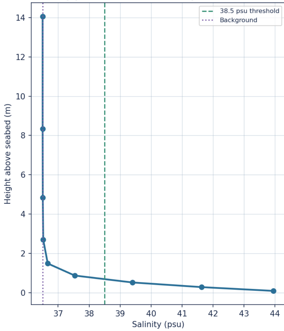
Figure. Vertical salinity profile at mid ebb - neap (saturated cavern brine)
