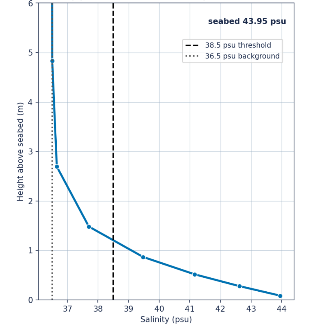
Vertical salinity profile at low water - neap (saturated cavern brine)
