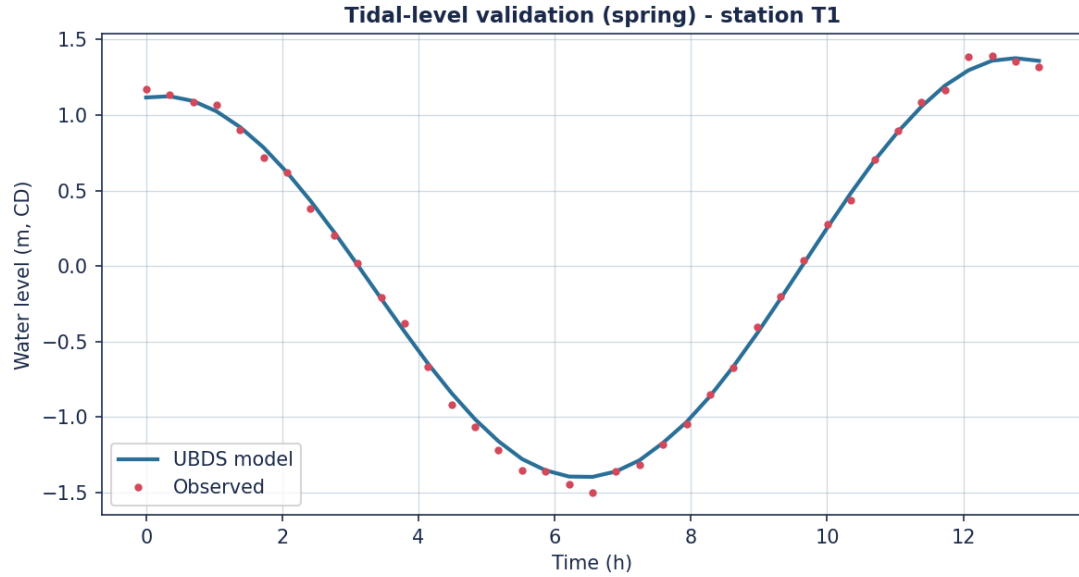
Figure. Modelled vs observed tidal level (spring tide) at the calibration station.
