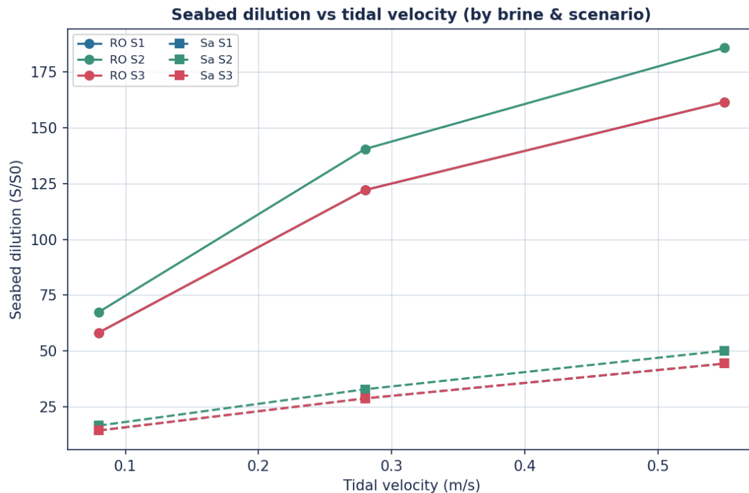
Figure. Seabed dilution as a function of tidal velocity for each brine type and scenario.
