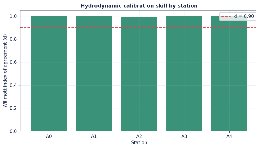
Figure. Index-of-agreement between modelled and observed currents by station (spring).
