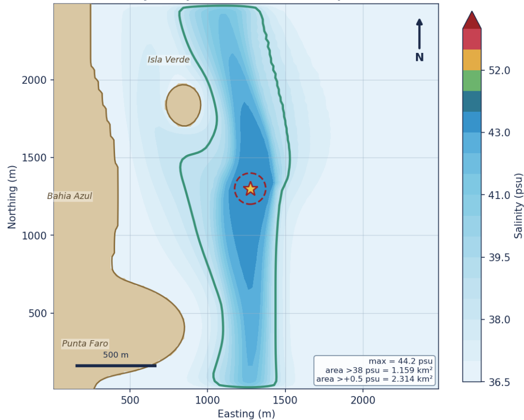
Maximum seabed salinity - 4-layer model (full flow, neap, saturated cavern brine)
