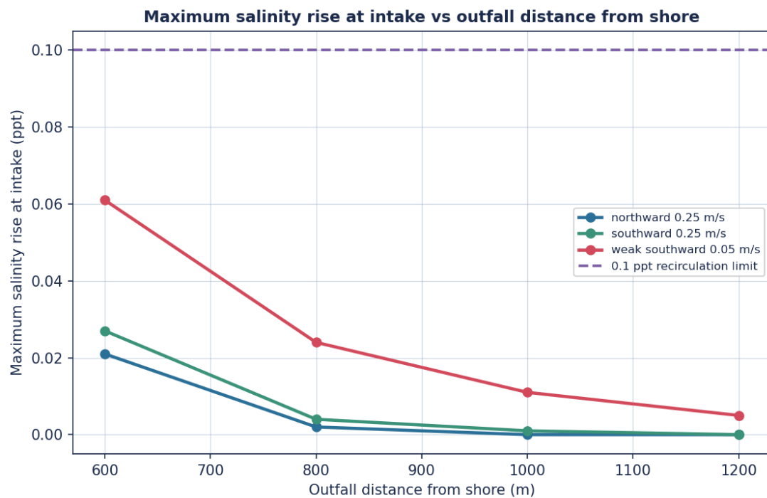
Figure. Variation of the maximum salinity rise at the intake with outfall distance from shore (recirculation criterion).
