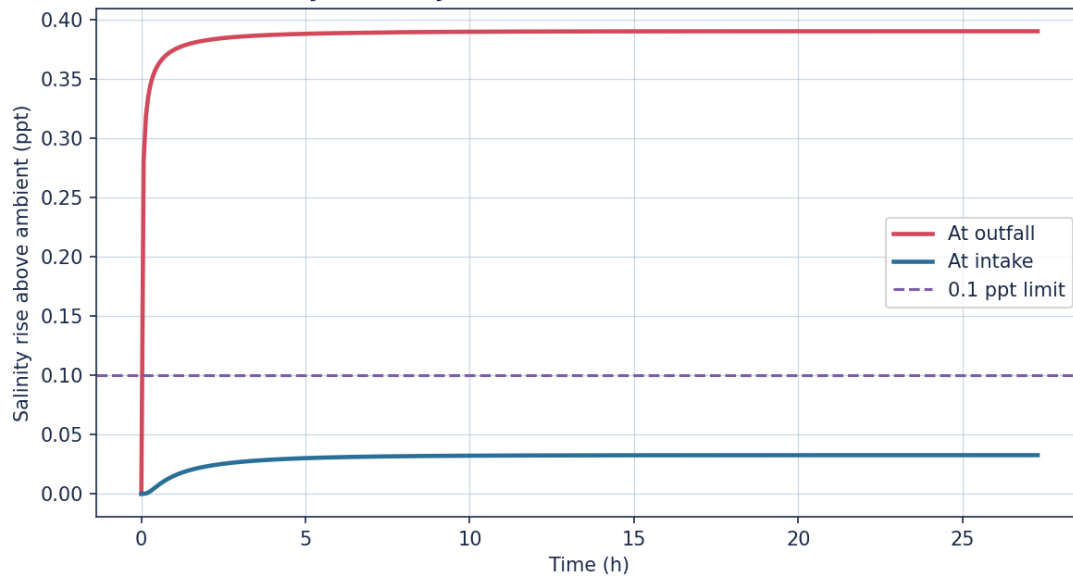
Time history of salinity rise - outfall 600 m from shore (weak current)
