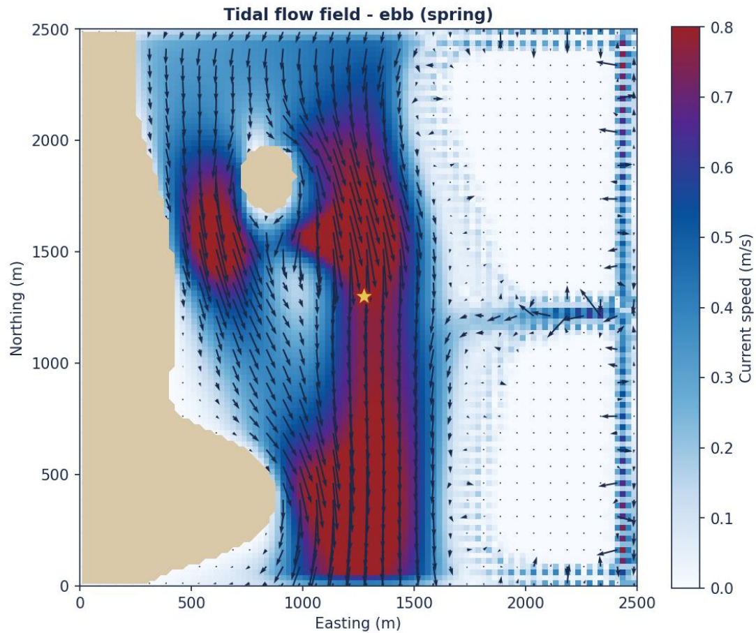
Figure. Depth-averaged tidal flow field at ebb (spring tide).
